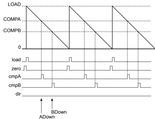
Figure 23-3. PWM Count-Down Mode
