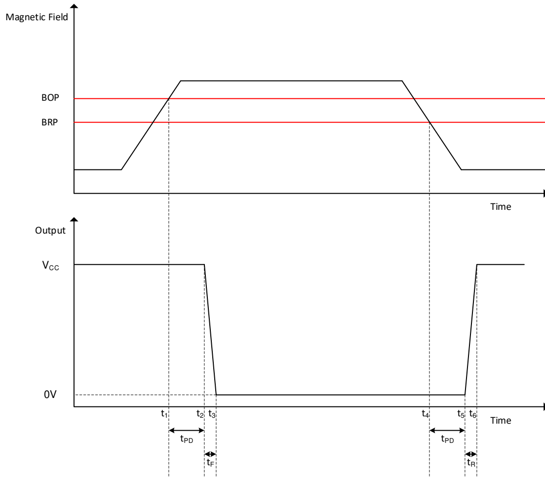
图 7-22. Propagation Delay
