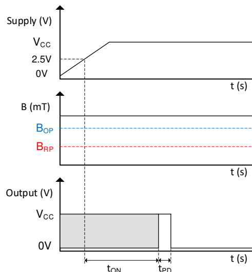
☒ 7-18. Power-On Time When B > B_{OP}
