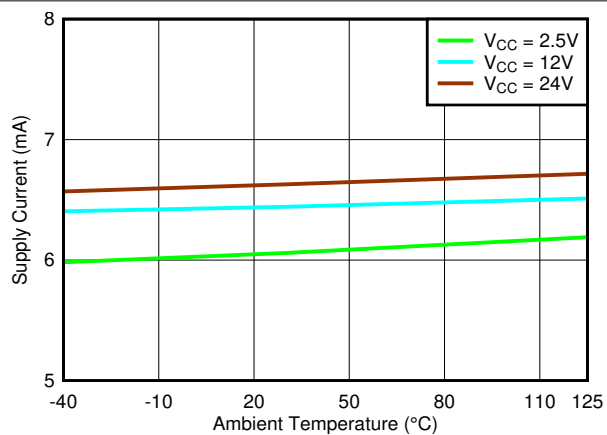
図 6-76. Supply Current vs Temperature
