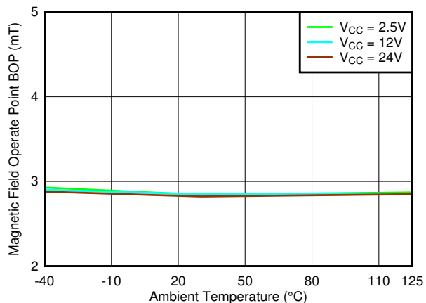
図 6-46. B OP_X Threshold vs Temperature
