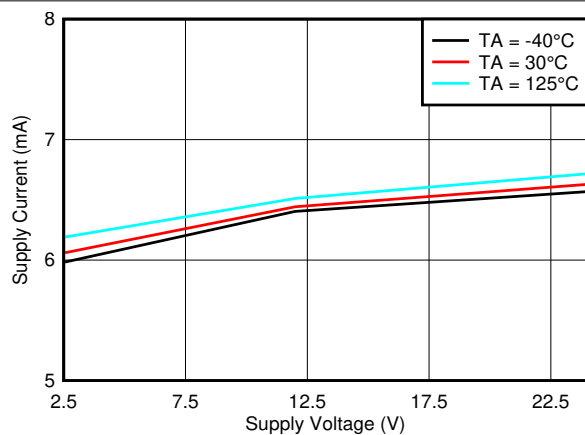
図 6-75. Supply Current vs V_{CC}
