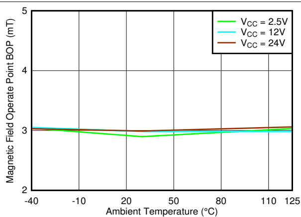
Figure 6-40. B OP_Z Threshold vs Temperature
