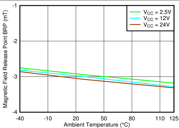
図 6-48. B RP_X Threshold vs Temperature
