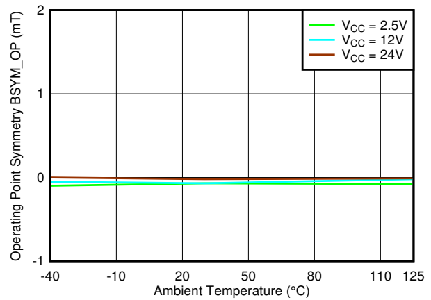
図 6-34. B_{SYM\_OP(XY)} vs Temperature
