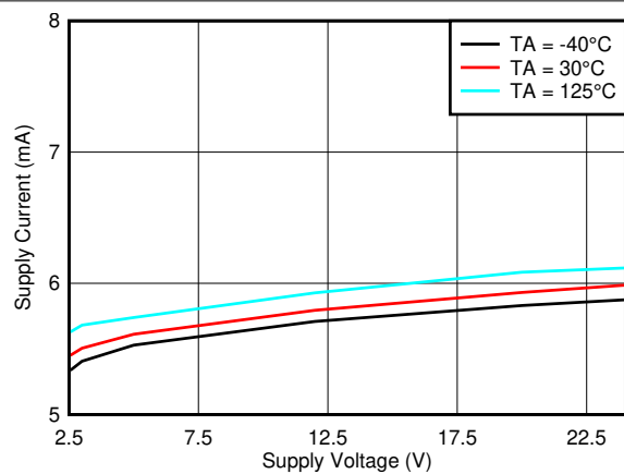
図 6-37. Supply Current vs V_{CC}
