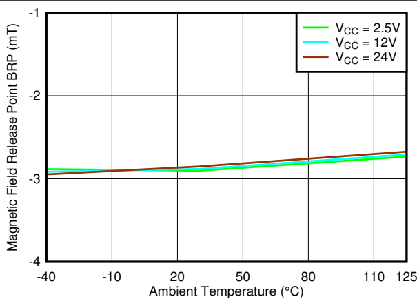
Figure 6-42. B RP_Z Threshold vs Temperature
