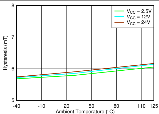
図 6-50. Hysteresis_X vs Temperature
