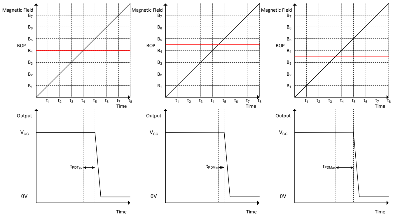
図 7-21. Field Sampling Timing
