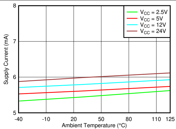
図 6-38. Supply Current vs Temperature
