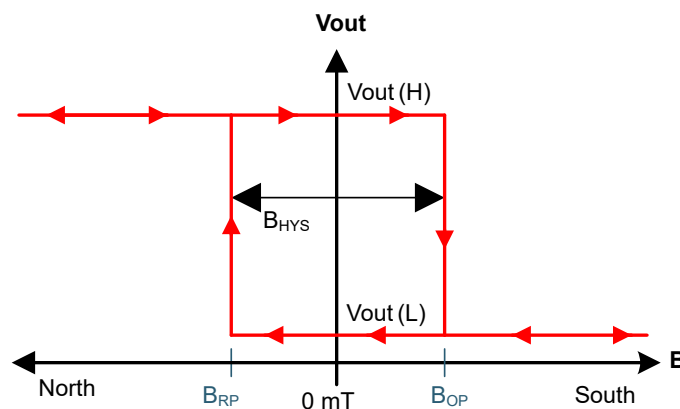
図 7-2. Latch Functionality
