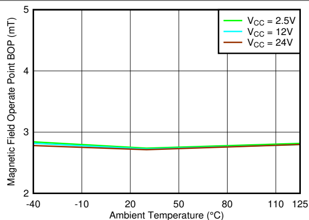
図 6-52. B OP_Y Threshold vs Temperature
