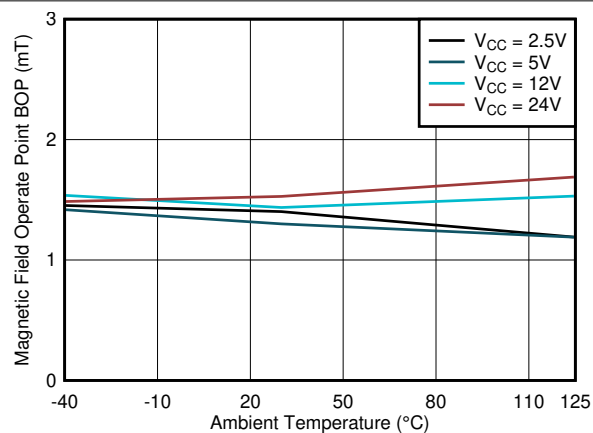
図 6-8. B_{OP\_X} Threshold vs Temperature
