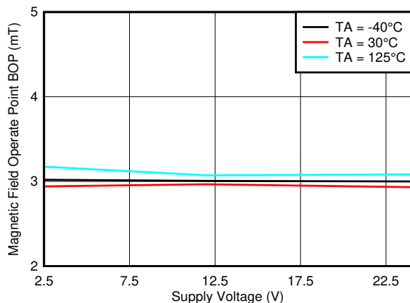
図 6-45. B OP_X Threshold vs V CC
