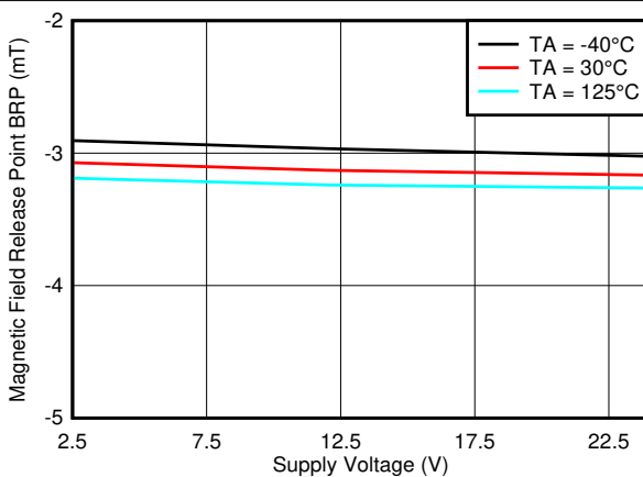
図 6-47. B RP_X Threshold vs V CC
