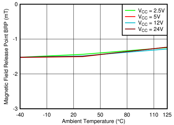
図 6-16. B RP_Y Threshold vs Temperature
