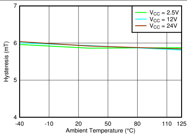
Figure 6-44. Hysteresis_Z vs Temperature
