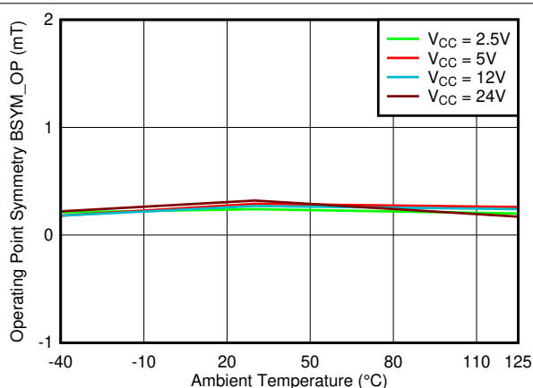
図 6-30. B_{SYM\_OP(ZY)} vs Temperature
