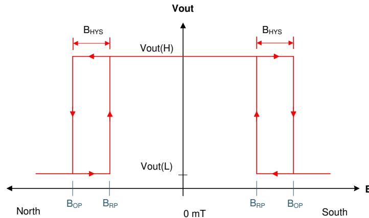
FIG 8-3. Omnipolar Functionality
