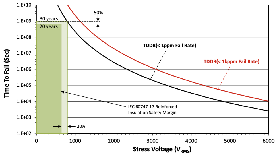
8-2. Insulation Lifetime
