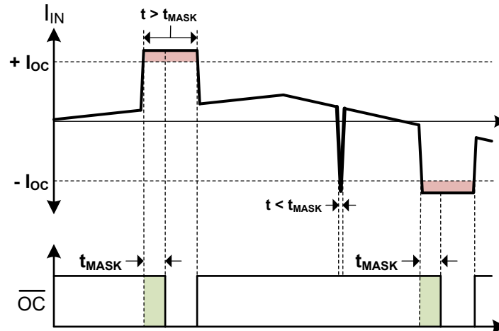
図 8-9. Overcurrent Detection MASK Diagram
