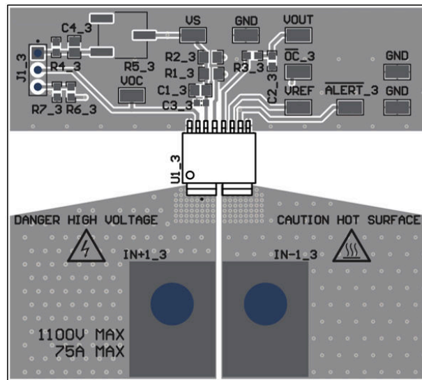
9-5. Recommended Board Layout
