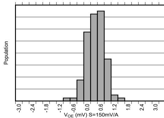
6-10. Offset Error Production Distribution
