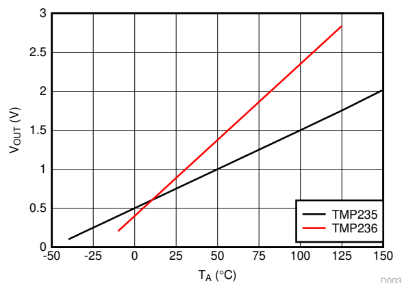
FIG 8-2. Output Voltage vs. Ambient
