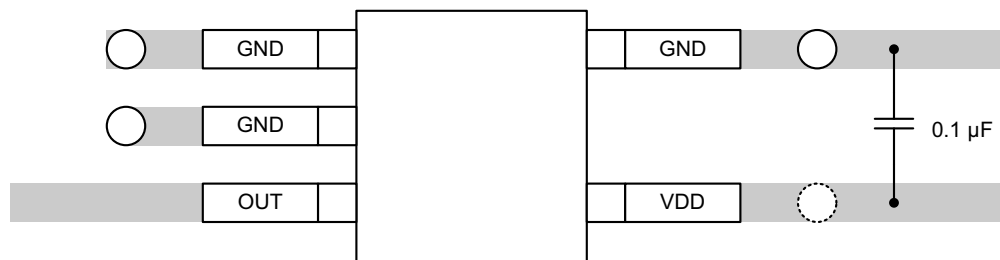
FIG 10-1. Recommended Layout: SC70 Package
