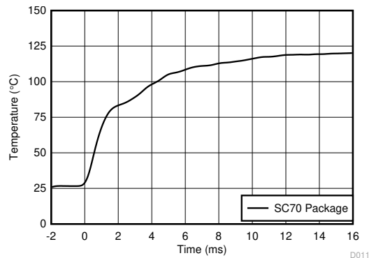
FIG 6-8. Thermal Response (Air-to-Fluid Bath)
