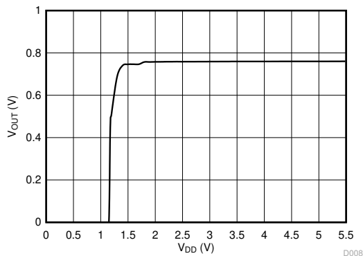
FIG 6-7. Output Voltage vs Power Supply
