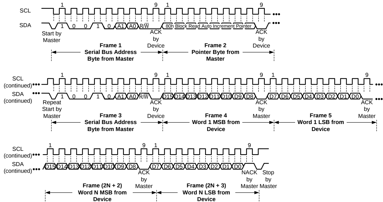
✎ 19. Two-Wire Timing Diagram for Pointer Byte Set Followed by a Repeat Start and Multiple-Word (N-Word) Read
