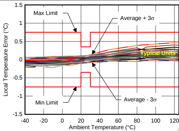
Typical behavior of 95 DSBGA devices over temperature at V_+ = 1.8\text{ V}
