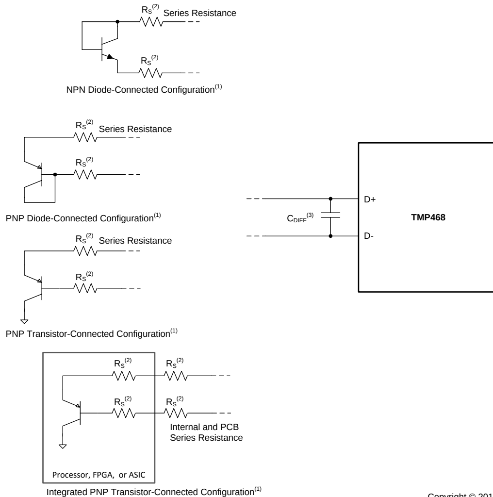
FIG 23. TMP468 Remote Transistor Configuration Options
