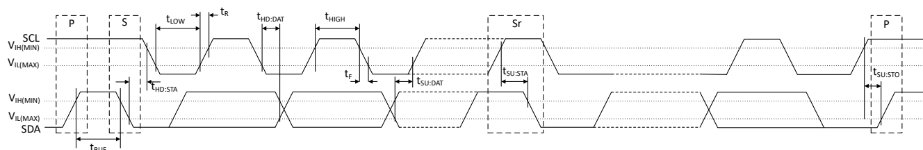
FIG 6-1. Two-Wire Timing Diagram
