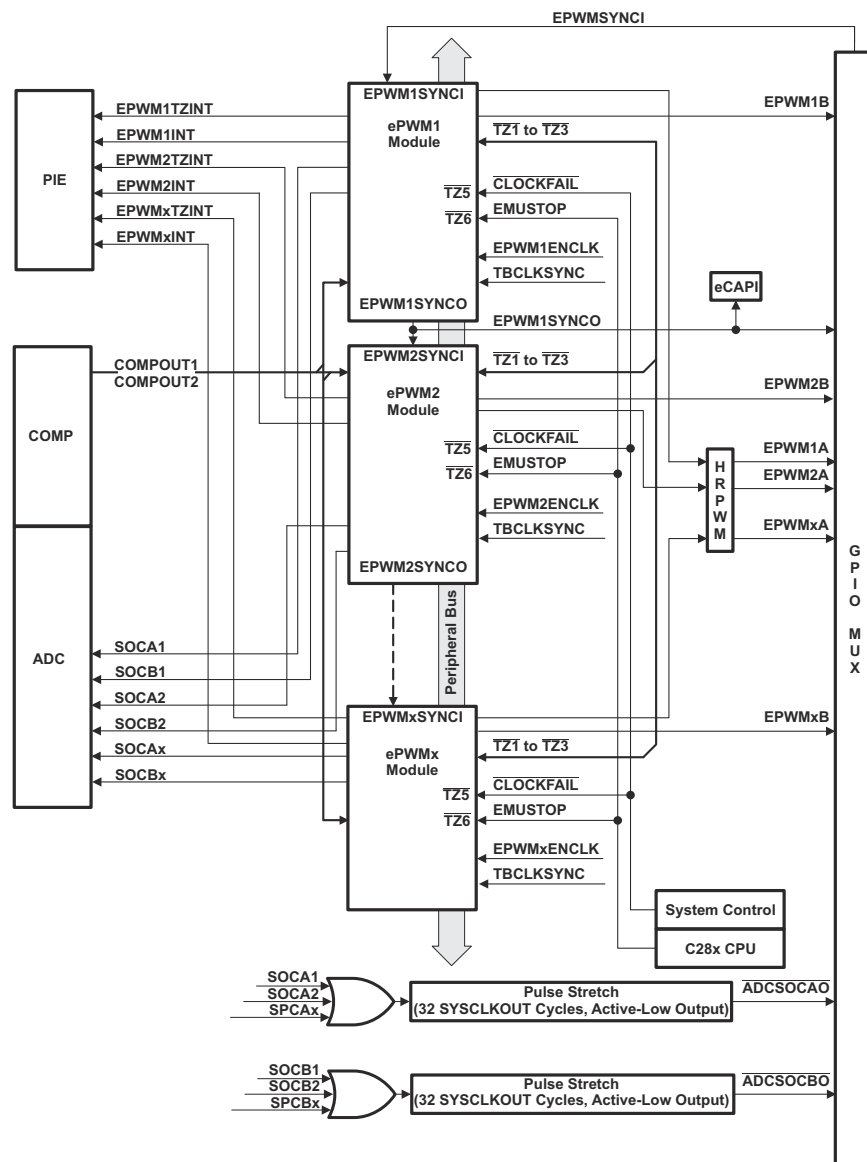
9-35. ePWM
