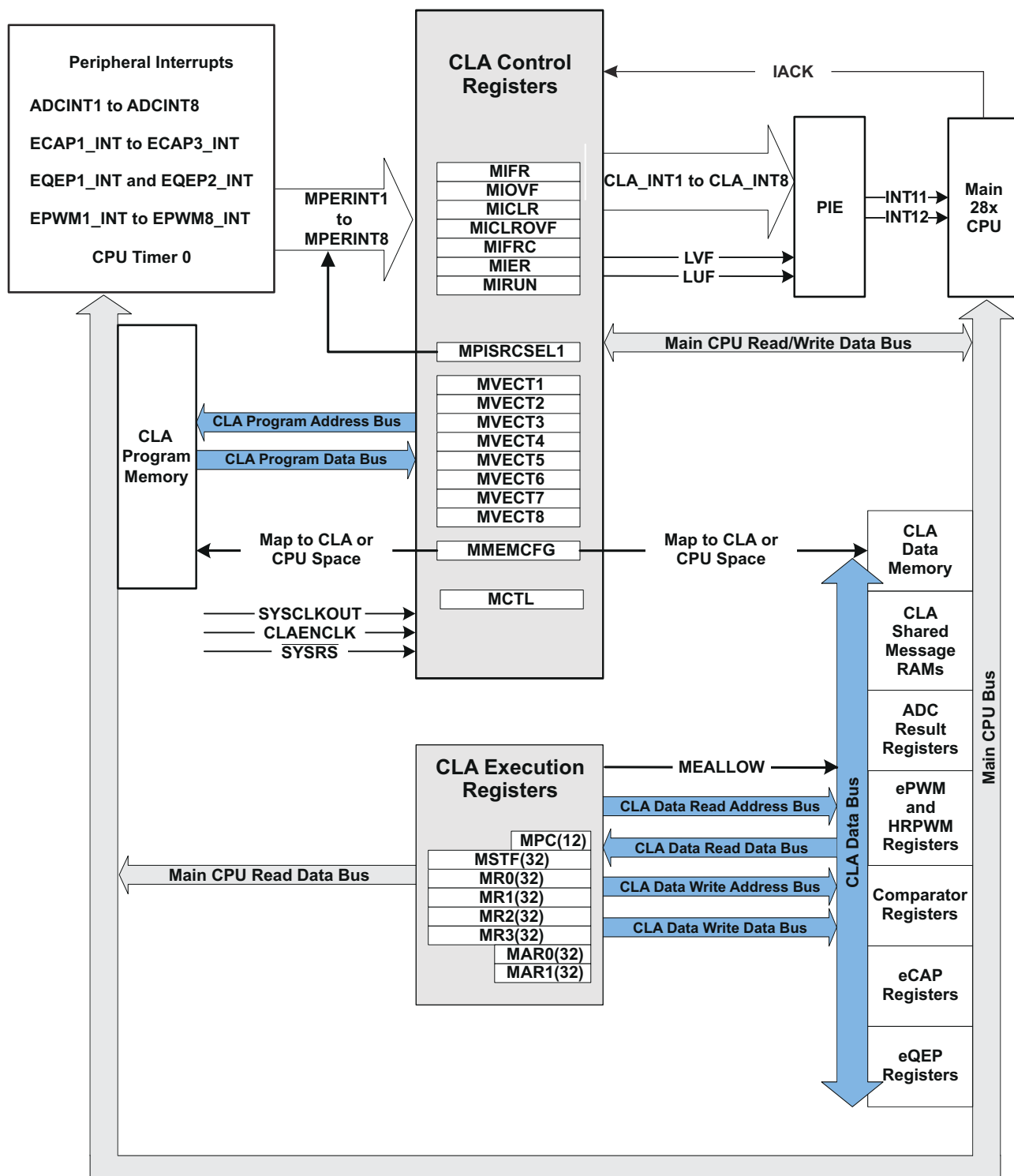
8-19. CLA Block Diagram
