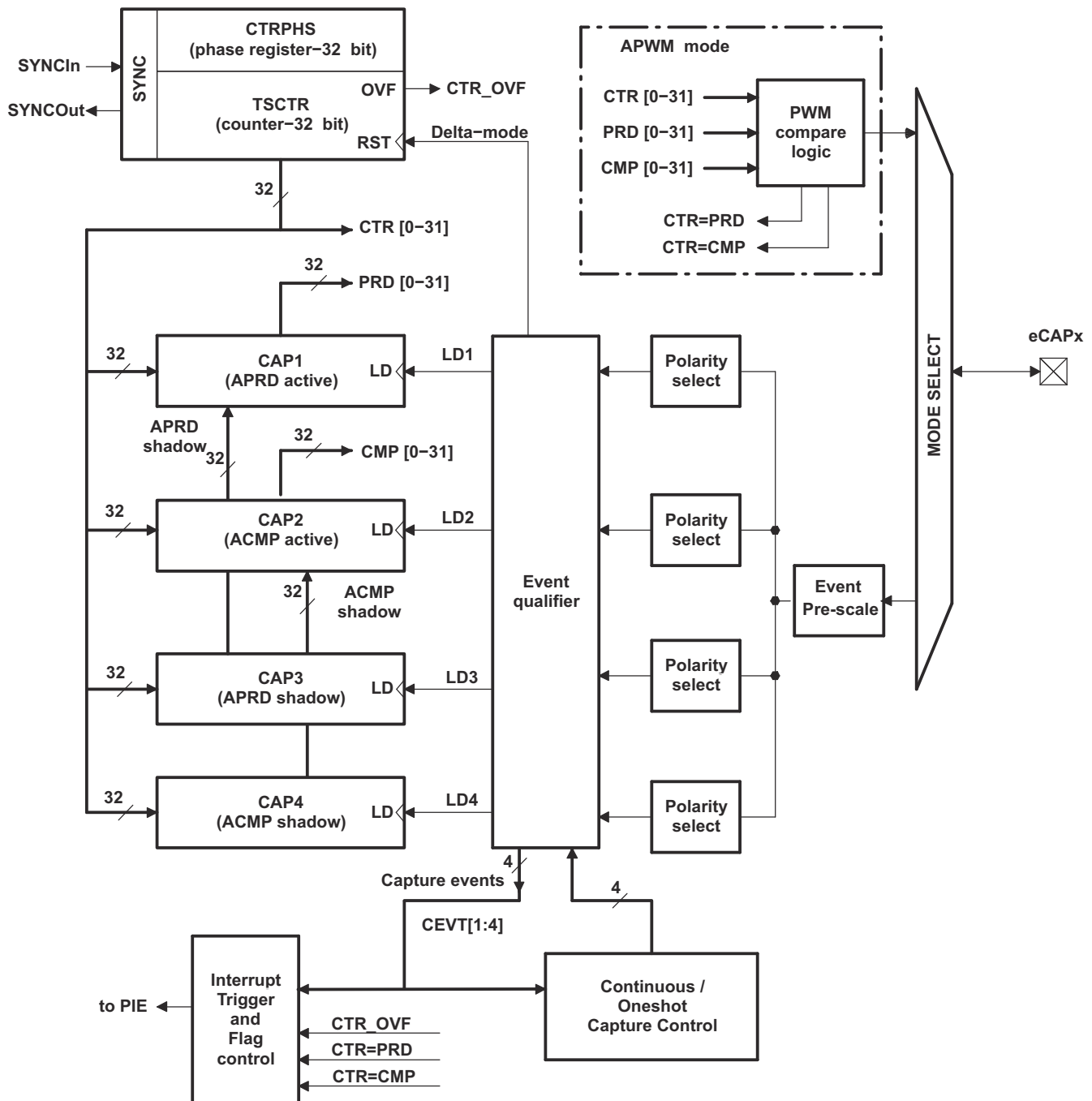
8-51. eCAP Functional Block Diagram
