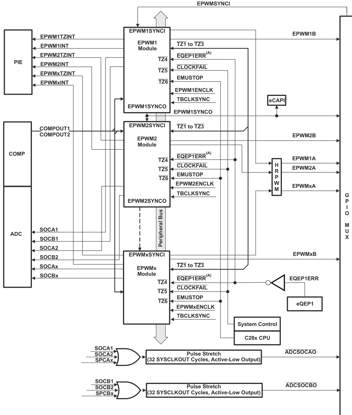
Figure 8-48. ePWM
