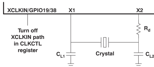
図 8-12. Using the On-chip Crystal Oscillator
