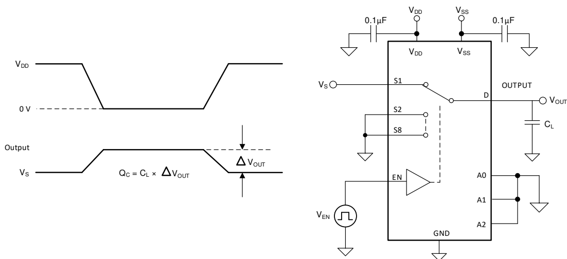
7-7. Charge-Injection Measurement Setup
