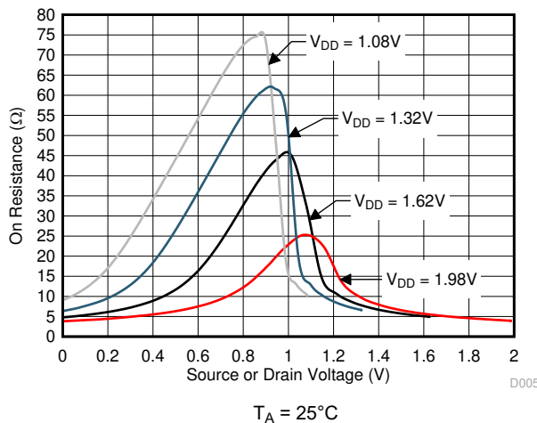
図 6-5. On-Resistance vs Source or Drain Voltage
