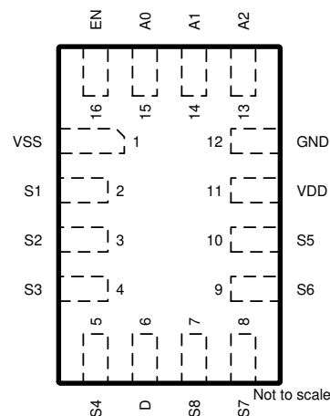
図 5-2. TMUX1108: RSV Package, 16-Pin QFN (Top View)
