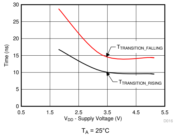
図 6-16. T_{TRANSITION} vs Supply Voltage
