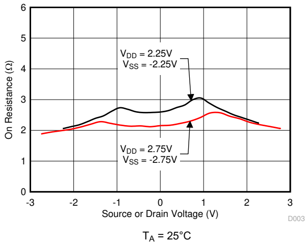
図 6-3. On-Resistance vs Source or Drain Voltage
