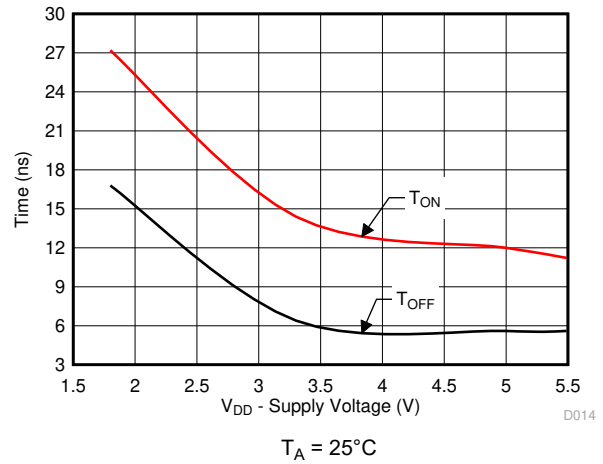
図 6-14. T_{ON} (EN) and T_{OFF} (EN) vs Supply Voltage
