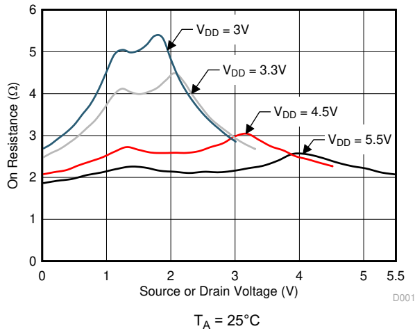
図 6-1. On-Resistance vs Source or Drain Voltage
