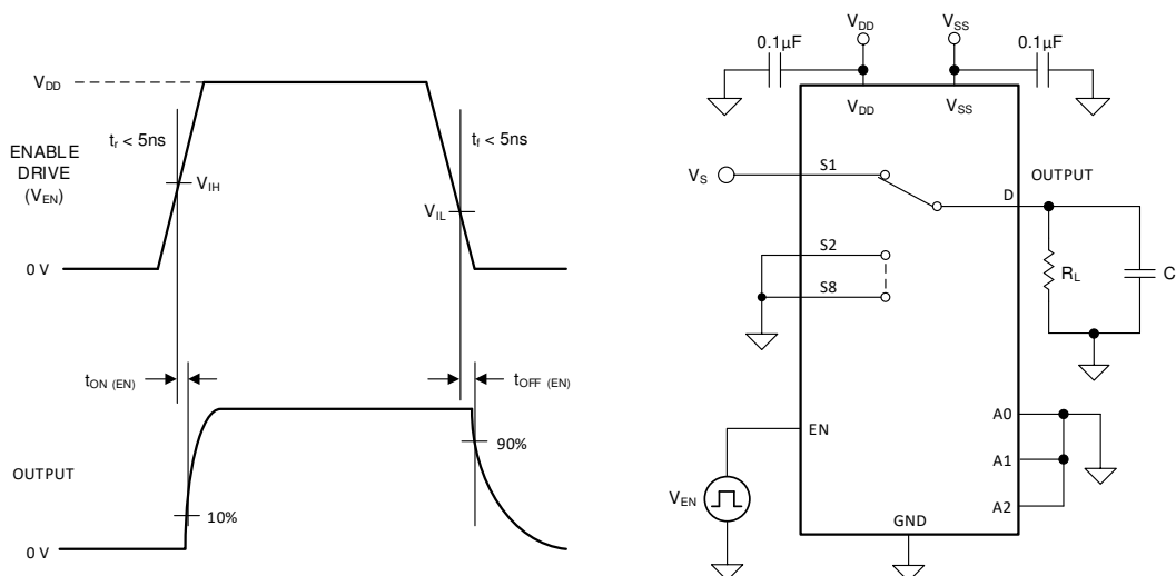
図 7-6. Turn-On and Turn-Off Time Measurement Setup
