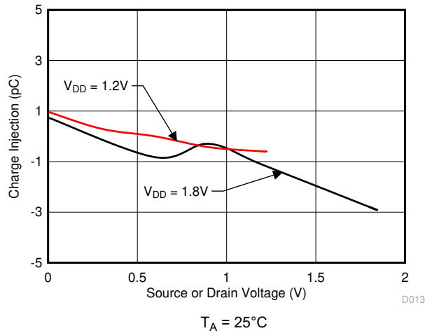
図 6-13. Charge Injection vs Source or Drain Voltage
