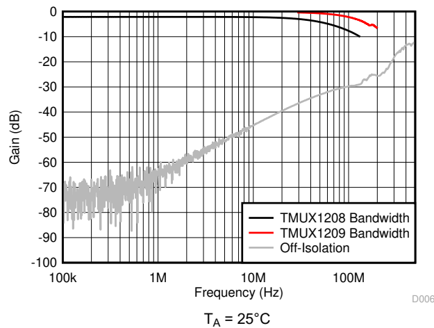
図 6-17. Frequency Response
