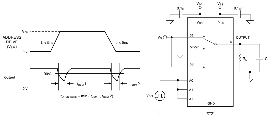
図 7-5. Break-Before-Make Delay Measurement Setup
