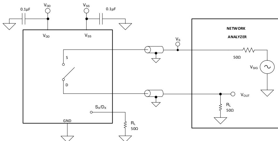
7-8. Off Isolation Measurement Setup
