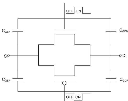
8-2. Transmission Gate Topology
