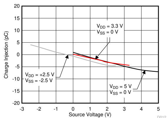
8-3. Charge Injection vs Source Voltage
