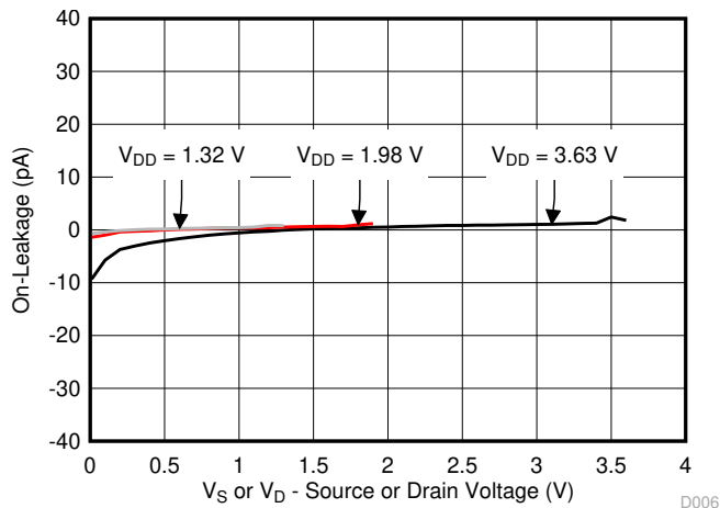
8-1. Leakage Current vs Input Voltage
