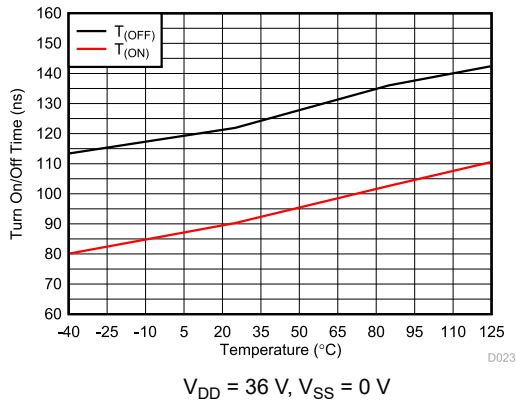
図 6-19. T_{ON} and T_{OFF} vs Temperature
