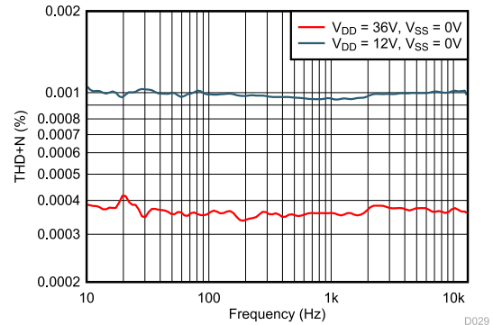
図 6-24. THD+N vs Frequency (Single Supplies)
