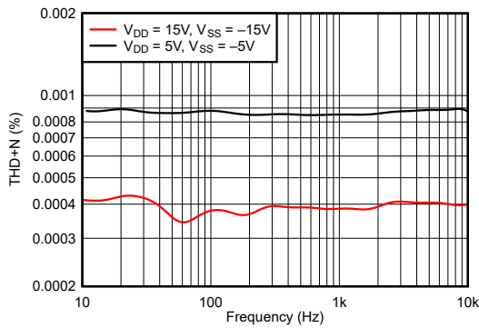
図 6-23. THD+N vs Frequency (Dual Supplies)
