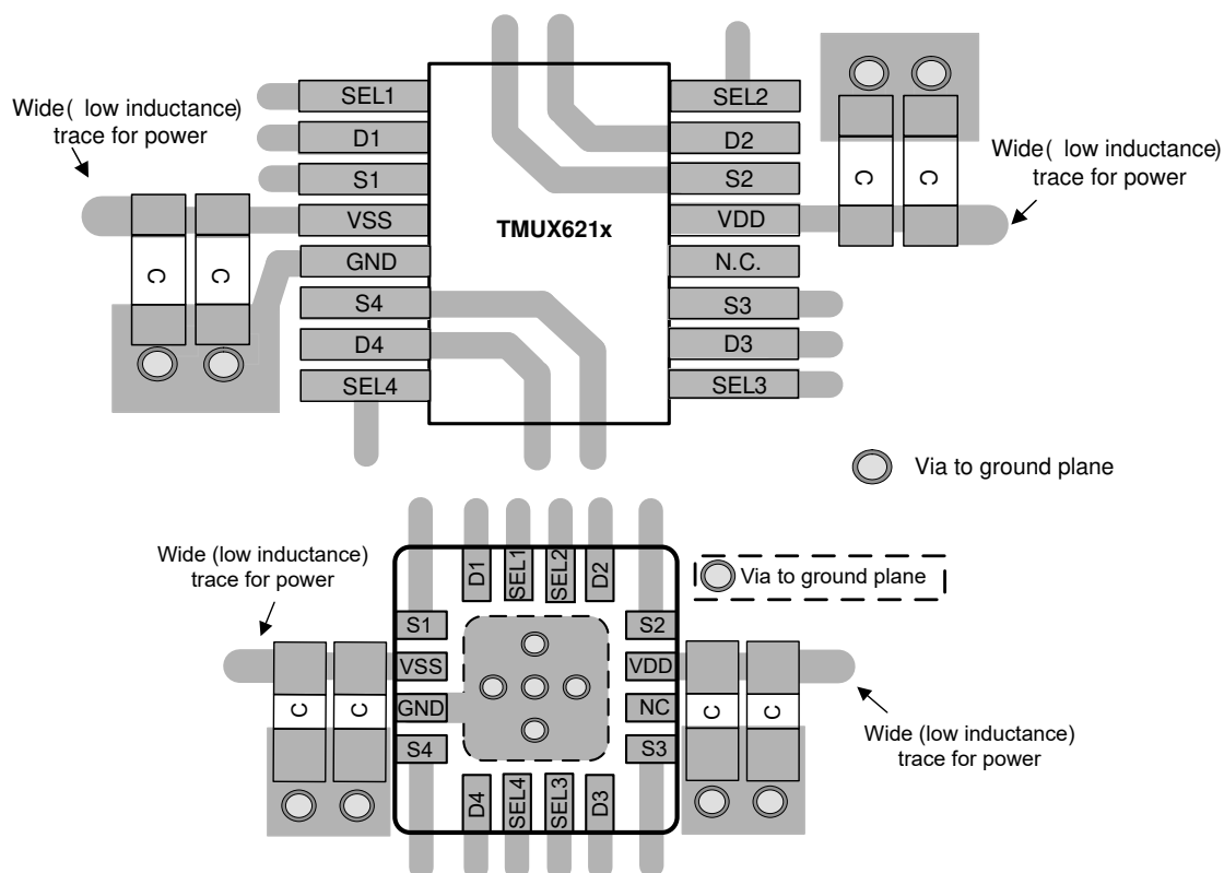
9-5. TMUX621x Layout Example
