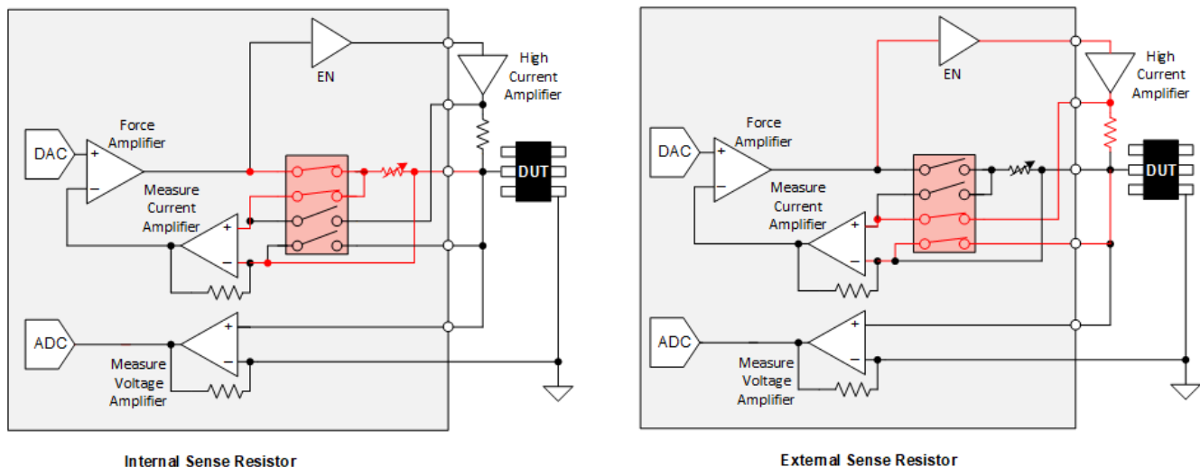
図 9-1. High Current Range Selection Using External Resistor
