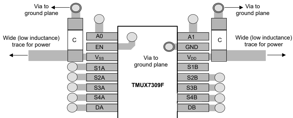
10-5. TMUX7309FPW Layout Example
