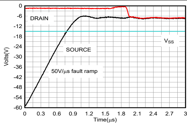
7-38. Drain Output Response – Negative Overvoltage
