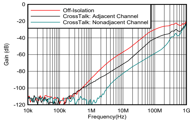
7-31. Off Isolation and Crosstalk vs Frequency
