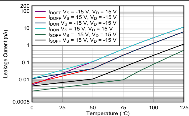
7-16. Leakage Current vs Temperature
