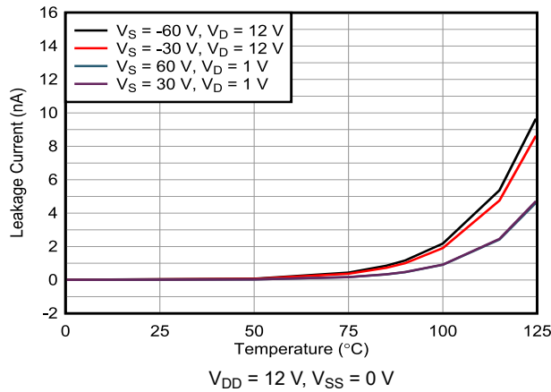
7-21. I_{D(FA)} Overvoltage Leakage Current vs Temperature
