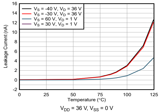
7-22. I_{D(FA)} Overvoltage Leakage Current vs Temperature
