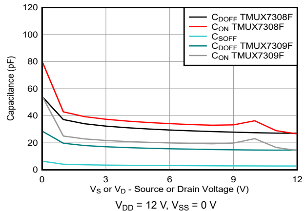
7-34. Capacitance vs Source or Drain Voltage
