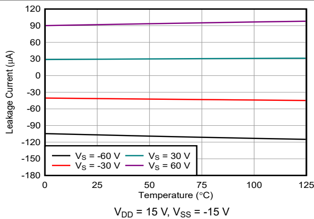
7-23. I_{S(FA)} Overvoltage Leakage Current vs Temperature
