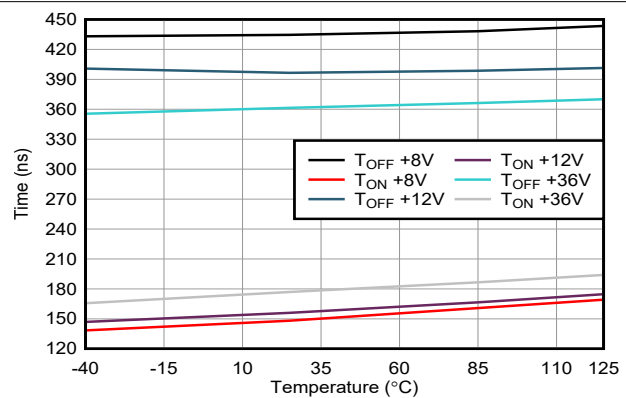
FIG 7-28. Transition Times vs Temperature
