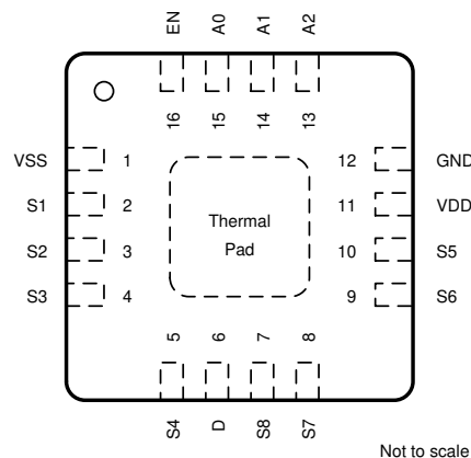
図 6-2. RRP Package, 16-Pin WQFN (Top View)
