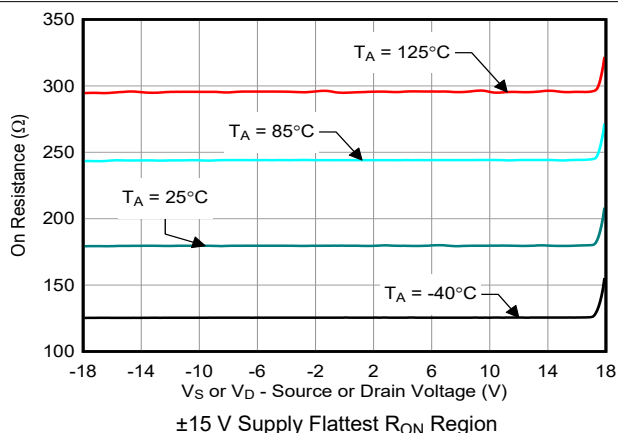
7-4. On-Resistance vs Source or Drain Voltage
