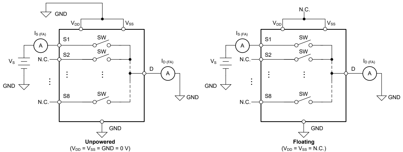
Figure 8-5. Measurement Setup for Input and Output Leakage Current under Overvoltage Fault with Unpowered or Floating Supplies
