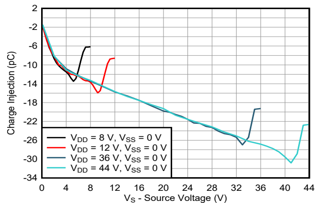
FIG 7-26. Charge Injection vs Source Voltage – Single Supply
