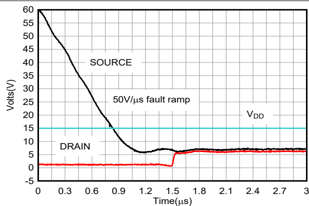
7-37. Drain Output Response – Positive Overvoltage
