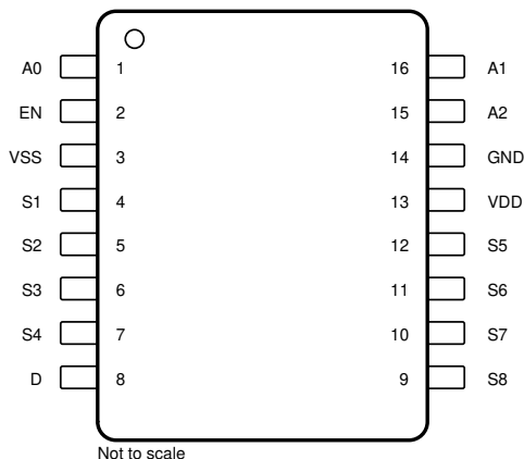
図 6-1. PW Package, 16-Pin TSSOP (Top View)
