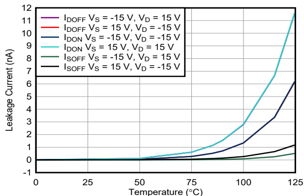
7-14. Leakage Current vs Temperature
