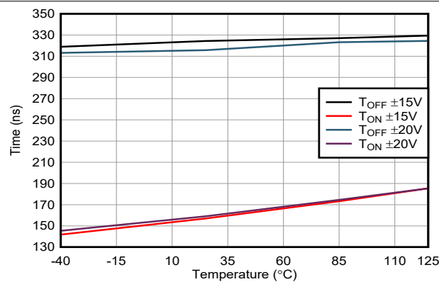
FIG 7-27. Transition Times vs Temperature
