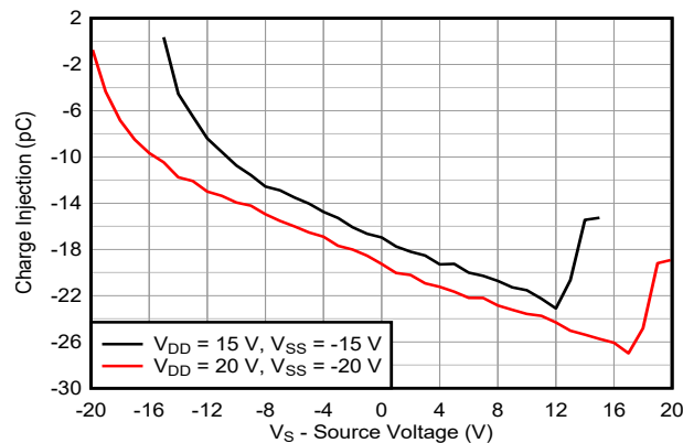
FIG 7-25. Charge Injection vs Source Voltage – Dual Supply
