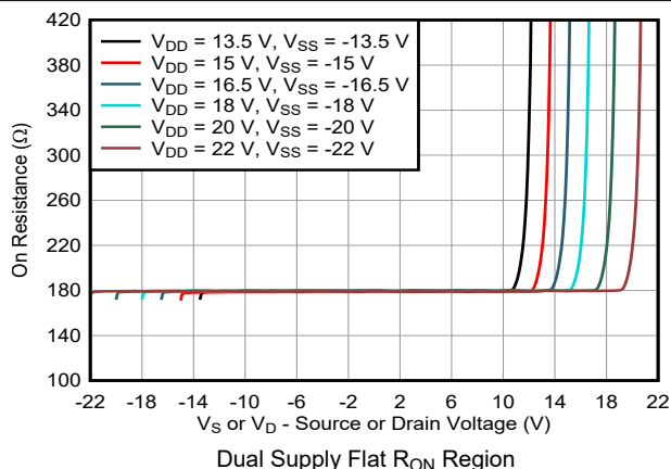
7-2. On-Resistance vs Source or Drain Voltage
