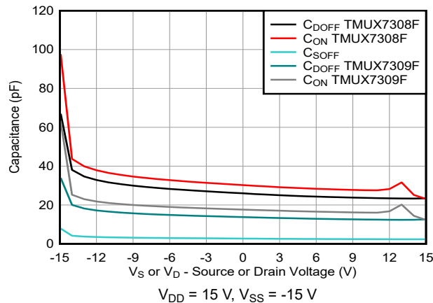
7-33. Capacitance vs Source or Drain Voltage
