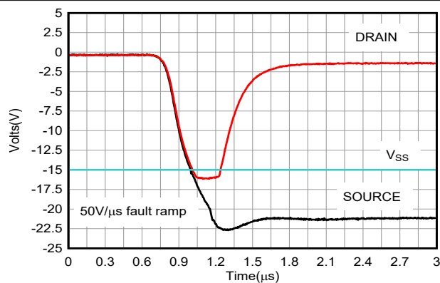
7-38. Drain Output Response – Negative Overvoltage
