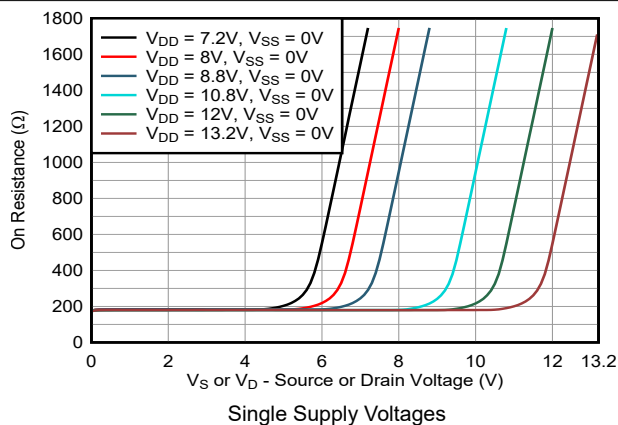
7-6. On-Resistance vs Source or Drain Voltage
