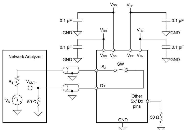
7-11. Bandwidth Measurement Setup
