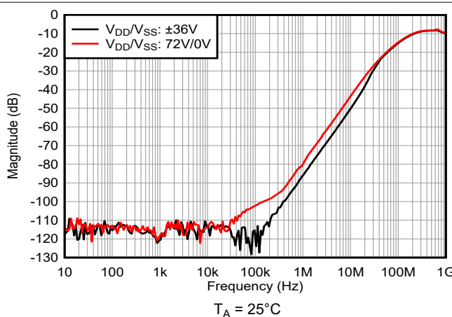
FIG 7-24. Off Isolation vs Frequency
