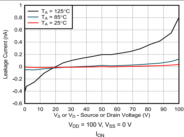
FIG 7-20. On-Leakage Current vs Source or Drain Voltage
