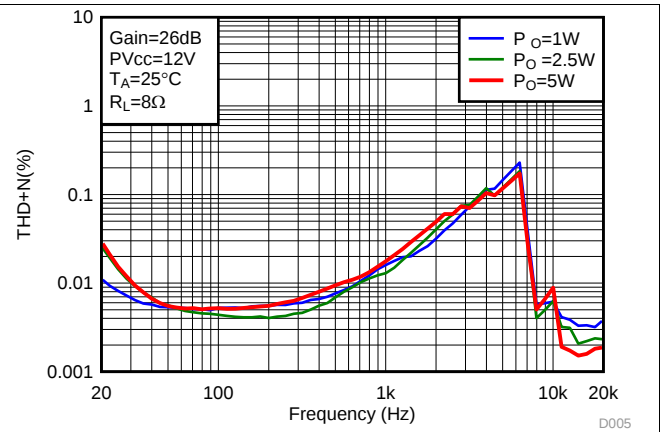
图 2. Total Harmonic Distortion + Noise (BTL) vs Frequency
