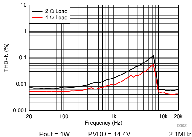
図 5-2. THD+N vs Frequency
