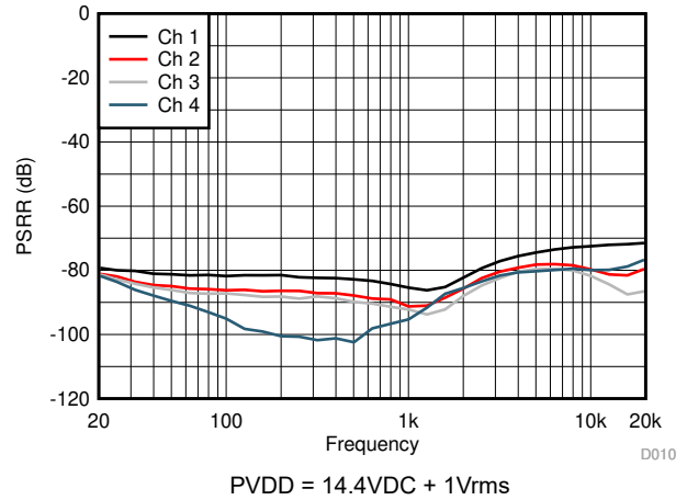
図 5-10. PVDD PSRR vs Frequency
