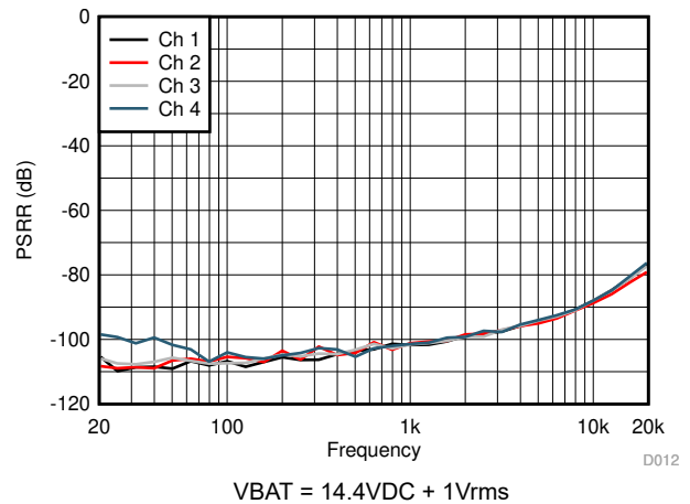
図 5-12. VBAT PSRR vs Frequency
