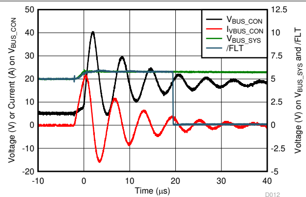
6-10. V_{BUS} Short-to-18 V Response Waveform
