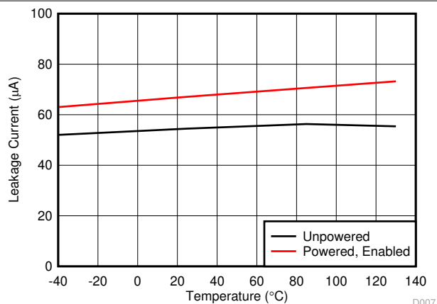
图 6-5. VD_{\pm} Leakage Current at 18-V across Temperature
