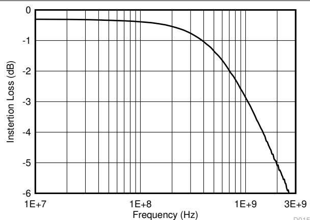
6-17. Data Switch Differential Bandwidth
