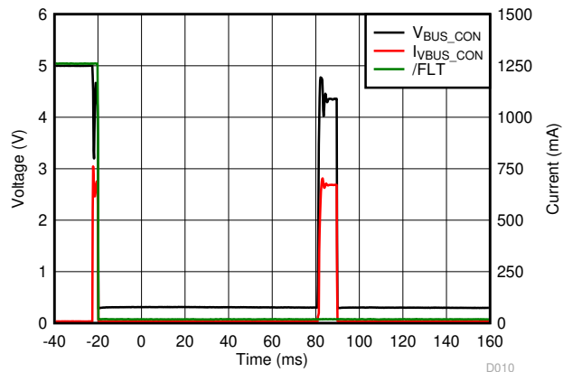
6-8. Overcurrent t_{BLANK\_RETRY} Response Waveform
