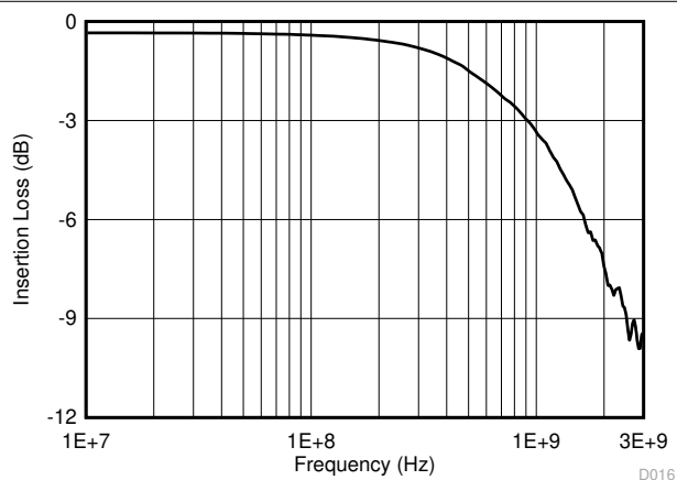
6-18. Data Switch Single-Ended Bandwidth
