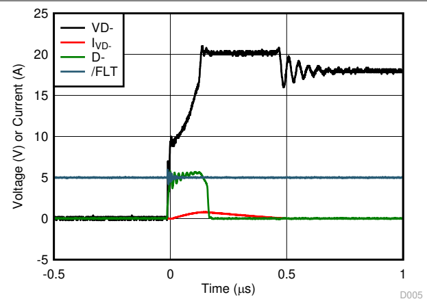
6-12. Data Switch Short-to-18 V Response Waveform
