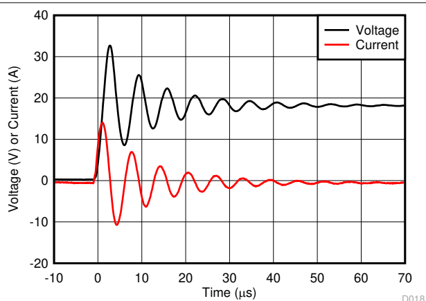
9-5. 100-V, 1-μF X7R Ceramic Shorted to 18 V
