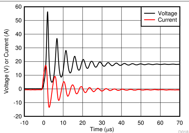
9-4. 50-V, 1-μF X7R Ceramic Shorted to 18-V (Not Recommended)
