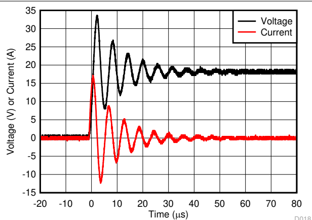
9-6. TPD3S716-Q1 and 100-V, 1-μF X7R Shorted to 18 V (Powered Off)
