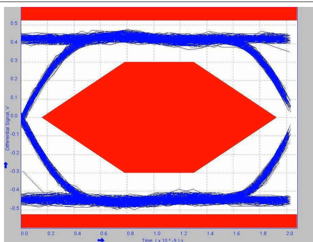
9-2. USB2.0 Eye Diagram (Board only, Through Path)
