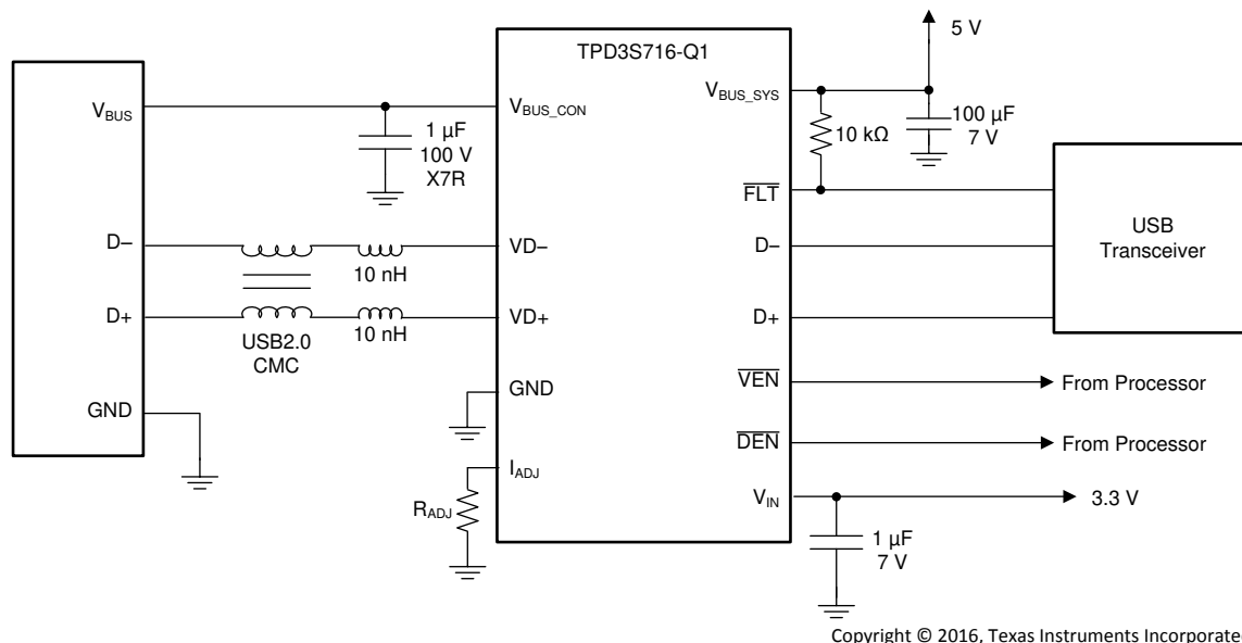
図 9-1. Typical Application Configuration for TPD3S716-Q1
