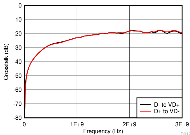
6-14. Data Switch Crosstalk
