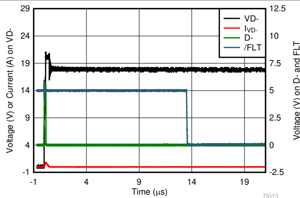
6-13. Data Switch Short-to-18 V Response Waveform (Long)
