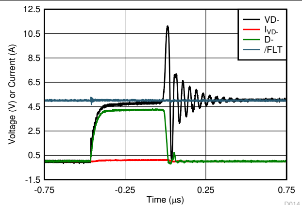
6-11. Data Switch Short-to-5 V Response Waveform
