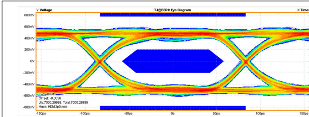
7-8. 6-Gbps HDMI 2.0 (TP1) Eye Diagram TPD4E05U06
