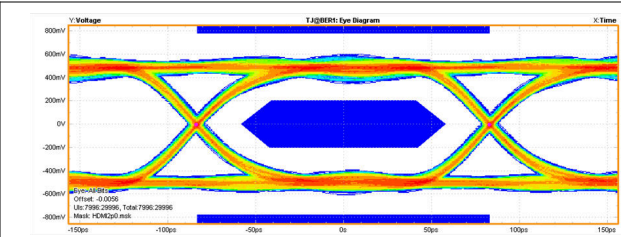
7-9. 6-Gbps HDMI 2.0 (TP1) Eye Diagram TPD6E05U06
