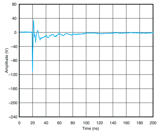
Figure 5-4. IEC Clamping Waveforms (-8-kV Contact)
