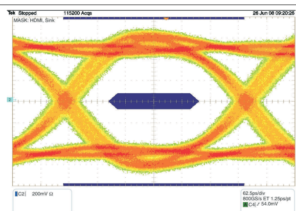
図 7-3. Eye Diagram With TPD8S009 (2.5Gbps Data Rate)
