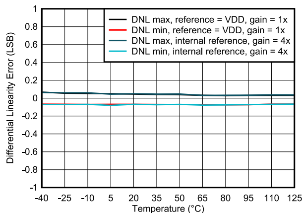
FIG 6-15. Differential Linearity Error vs Temperature
