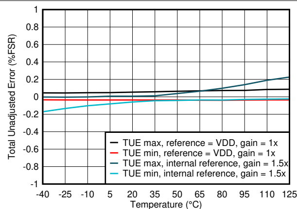
FIG 6-6. Total Unadjusted Error vs Temperature
