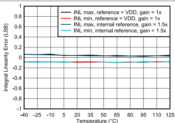
FIG 6-4. Integral Linearity Error vs Temperature
