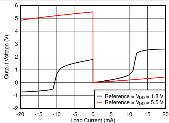
FIG 6-34. Source and Sink Capability
