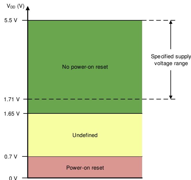
Figure 7-1. Threshold Levels for V_{DD} POR Circuit
