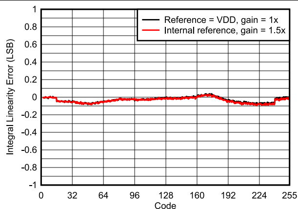
FIG 6-1. Integral Linearity Error vs Digital Input Code
