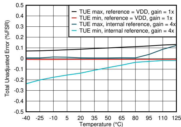
FIG 6-16. Total Unadjusted Error vs Temperature
