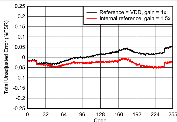
FIG 6-3. Total Unadjusted Error vs Digital Input Code
