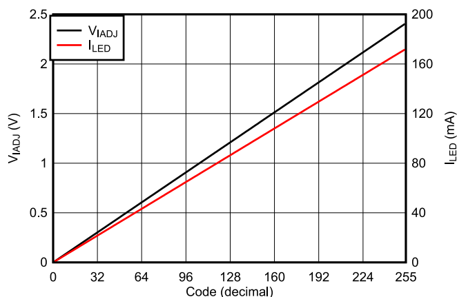
FIG 8-2. Digipot Code vs LED Current
