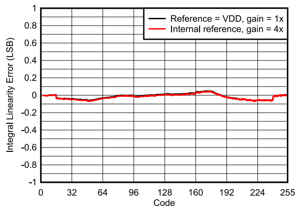
FIG 6-11. Integral Linearity Error vs Digital Input Code
