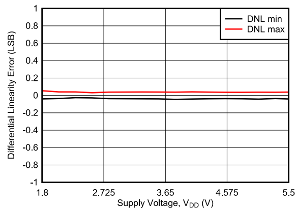
FIG 6-22. Differential Linearity Error vs Supply Voltage
