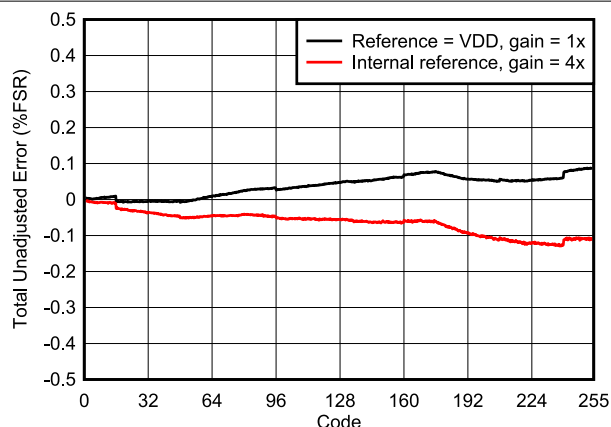
FIG 6-13. Total Unadjusted Error vs Digital Input Code
