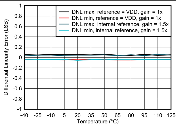
FIG 6-5. Differential Linearity Error vs Temperature
