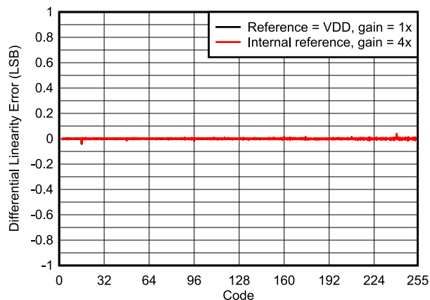
FIG 6-12. Differential Linearity Error vs Digital Input Code
