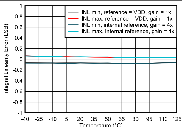
FIG 6-14. Integral Linearity Error vs Temperature
