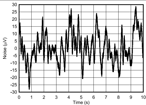
6-46. Digipot Output Noise: 0.1 Hz to 10 Hz
