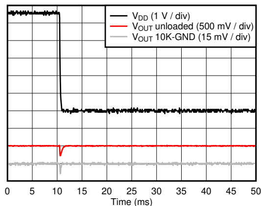
FIG 6-40. Power-off Glitch
