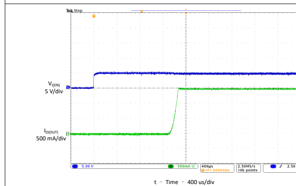
Figure 6-15. Short-Circuit Current, Device Enabled Into Short
