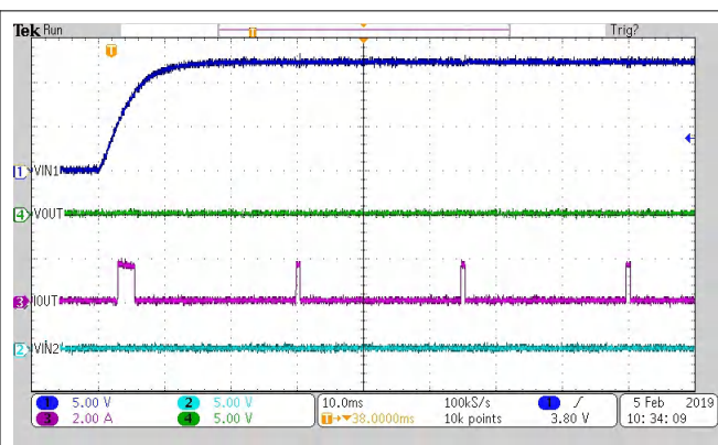
图 7-8. TPS2120 IN1 is Enabled with a Short on OUT
