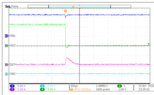
图 7-7. TPS2121 Hot Short on OUT while IN1 is Enabled
