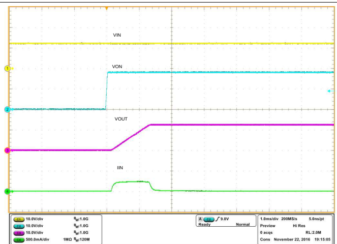
29. TPS22810-Q1 Inrush Current with C_L = 22 \mu F , CT = 4700 pF
