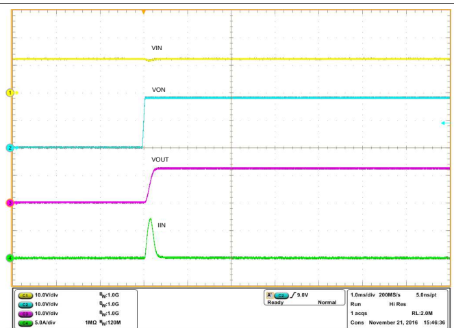
29. TPS22810-Q1 Inrush Current with C_L = 22 \mu F , CT = 4700 pF
