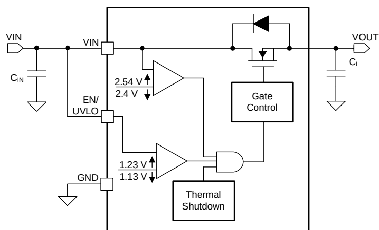
图 20. Default UVLO Threshold V_{UVL} Using No Additional External Components
