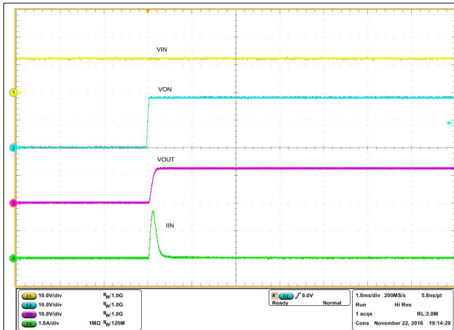
28. TPS22810-Q1 Inrush Current With C_L = 22 \mu F , CT = 0 pF
