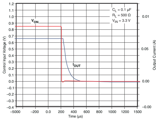
图 7-49. t_{OFF} Response
