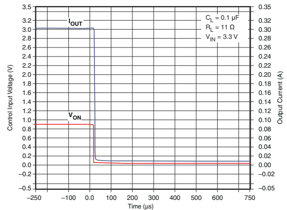
图 7-50. t_{OFF} Response
