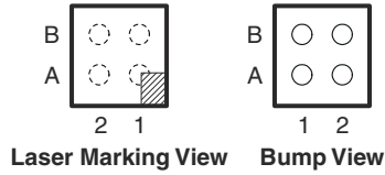
6-1. YFP Package 4-Pin DSBGA
