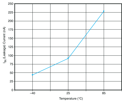
7-9. I_{IN} (Leakage) vs Temperature ( V_{IN} = 3.3 V)
