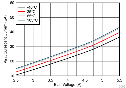
図 6-2. V_{BIAS} Quiescent Current vs Bias Voltage Single Channel (TPS22976, TPS22976N)
