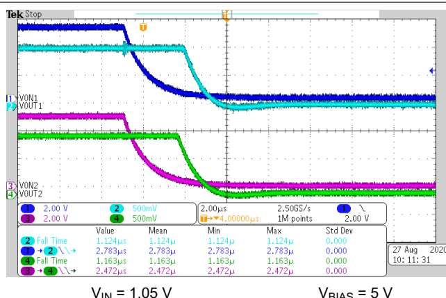
図 6-46. Turnoff Response Time
