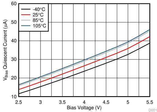
図 6-1. V_{BIAS} Quiescent Current vs Bias Voltage Both Channels (TPS22976, TPS22976N)
