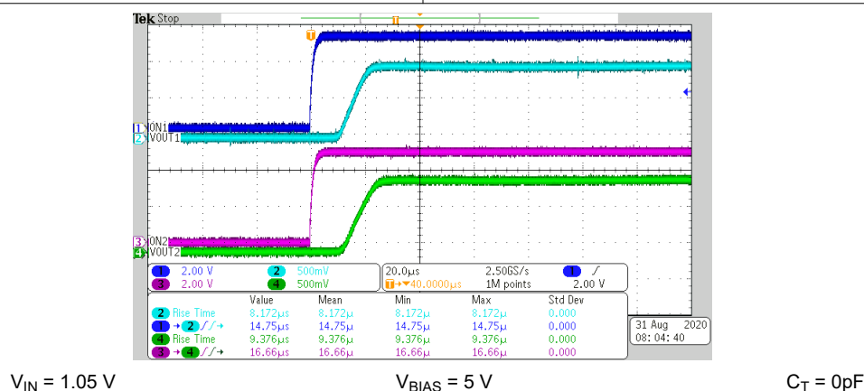
図 6-47. Turnon Response Time
