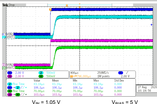
図 6-45. Turnon Response Time
