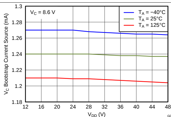
Figure 10. VC Bootstrap Current Source vs Supply Voltage
