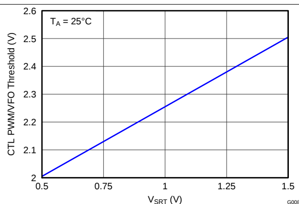
Figure 11. CTL PWM/VFO Threshold vs SRT Voltage
