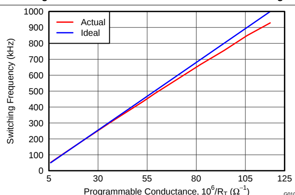
Figure 13. Switching Frequency vs Programmable Conductance
