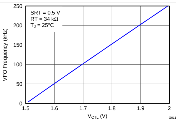
Figure 14. VFO Frequency vs CTL Voltage
