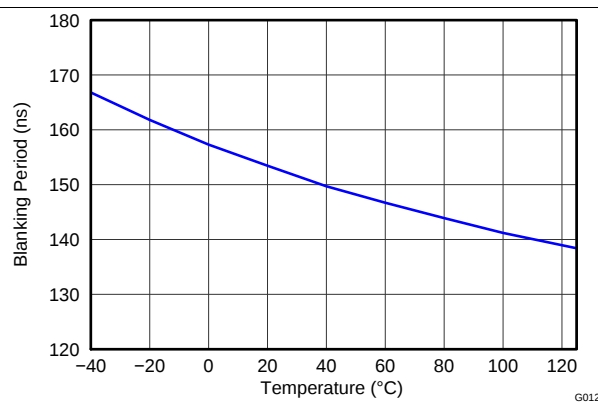
Figure 15. Blanking Period vs Temperature
