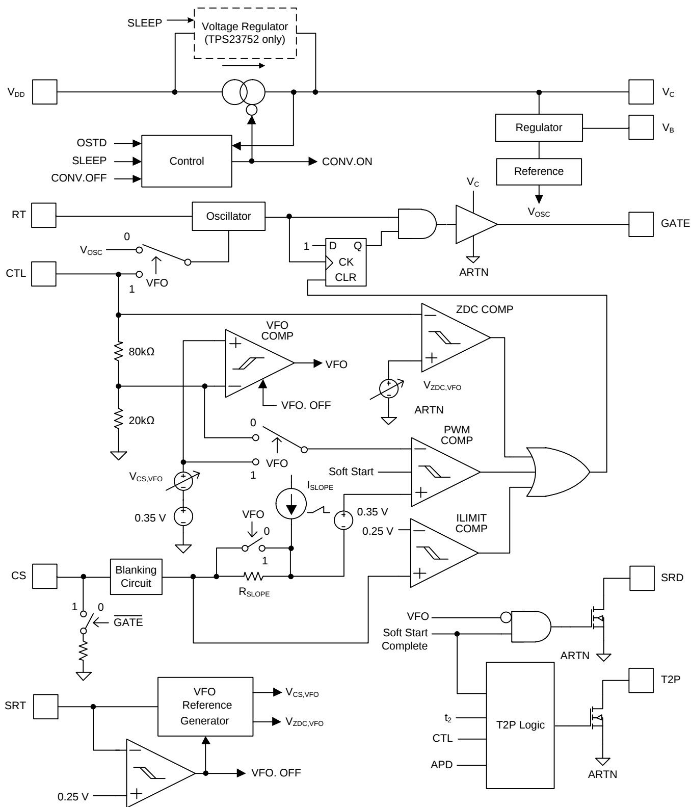
Figure 19. DC-DC Controller
