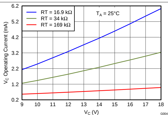
Figure 7. VC Operating Current vs VC Voltage
