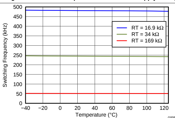
Figure 12. Switching Frequency vs Temperature
