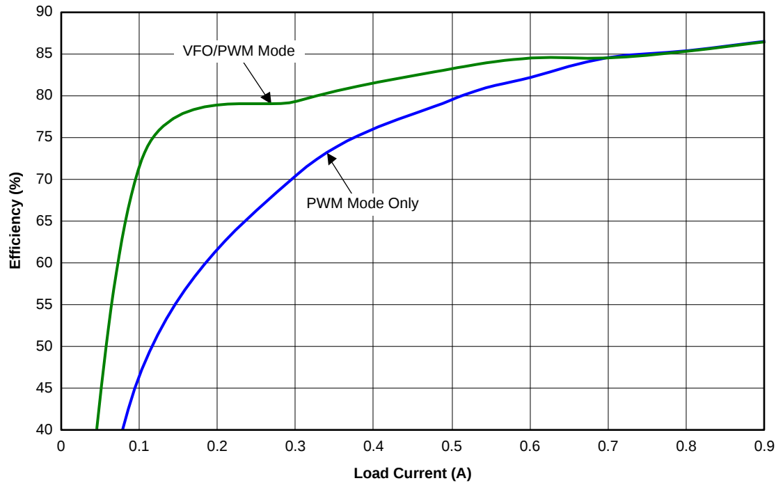
Figure 28. TPS23751 and TPS23752 Light Load Efficiency versus Mode
