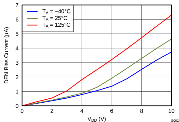
Figure 5. DEN Bias Current vs Supply Voltage
