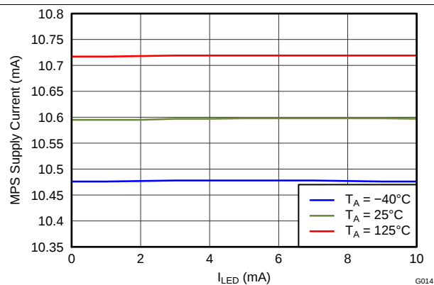
Figure 17. MPS Supply Current vs LED Current
