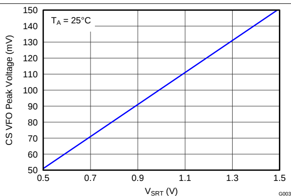
Figure 6. CS VFO Peak Voltage vs SRT Voltage
