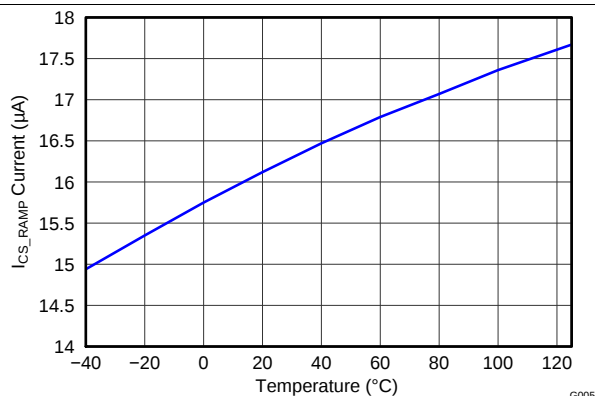
Figure 8. CS Ramp Current vs Temperature
