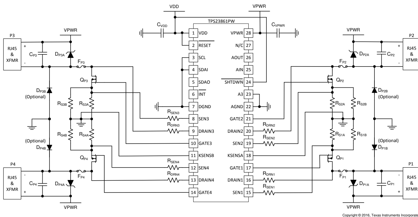
Figure 49. Four Port Auto Mode Application
