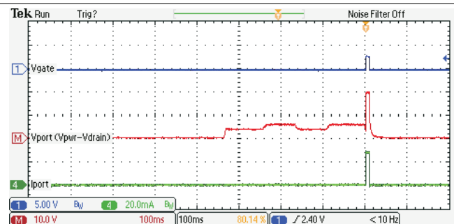
Figure 16. Classification Voltage vs Port Classification Current
