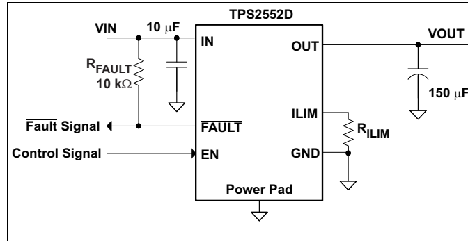
Figure 1. Typical Characteristics Reference Schematic
