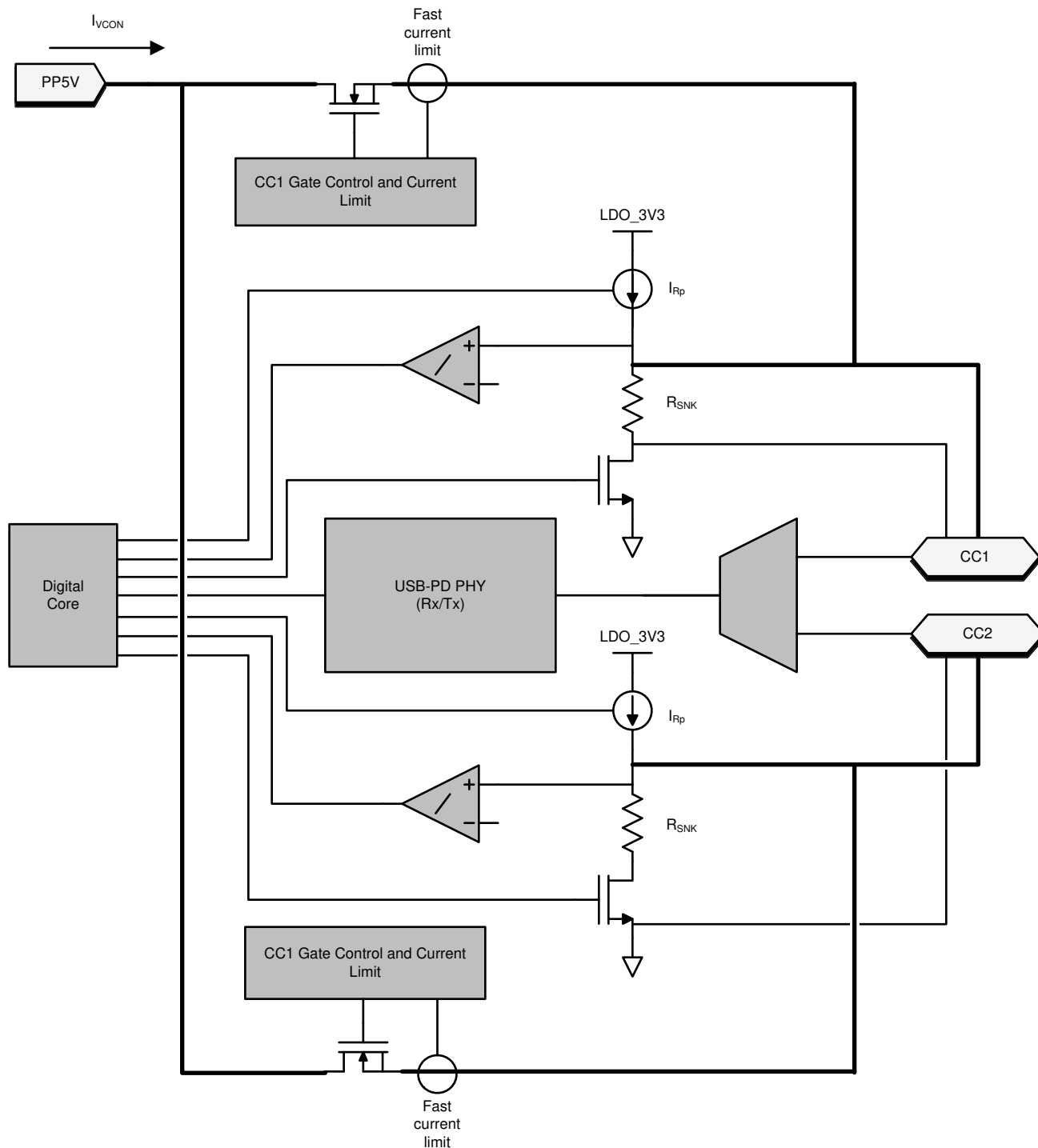
8-3. USB-PD Physical Layer and Simplified Plug and Orientation Detection Circuitry
