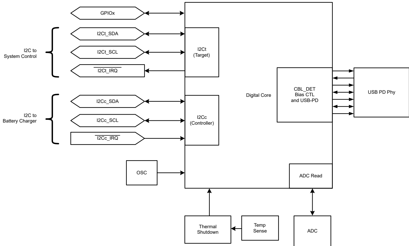
8-26. Digital Core Block Diagram
