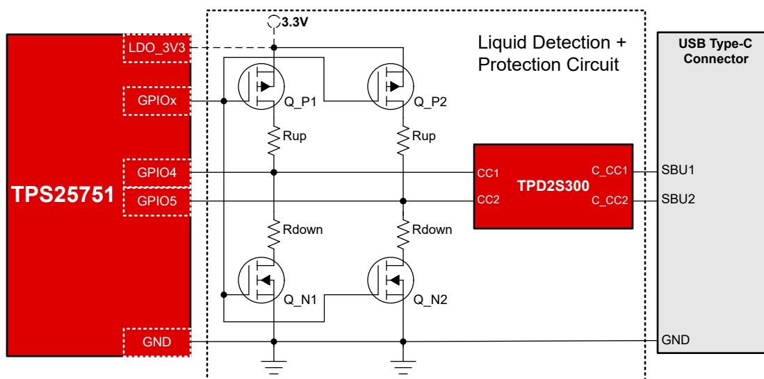
図 9-9. TPS25751 Liquid Detection Block Diagram - 1 GPIO Control
