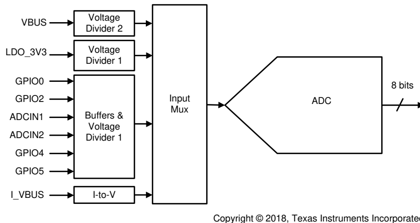
Figure 8-23. SAR ADC
