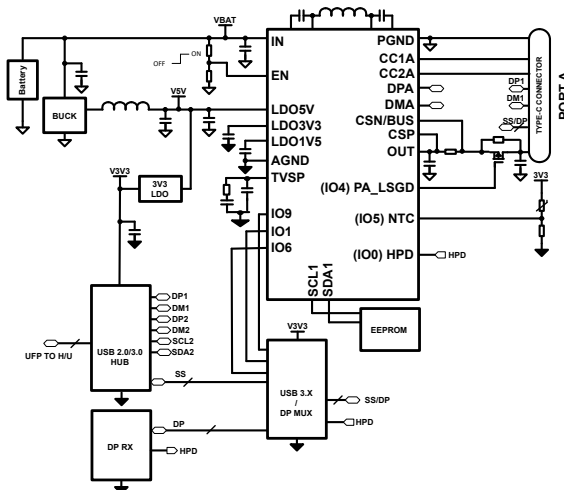
9-2. Simplified Single USB PD Charger with DisplayPort Alt Mode - MUX control with GPIO
