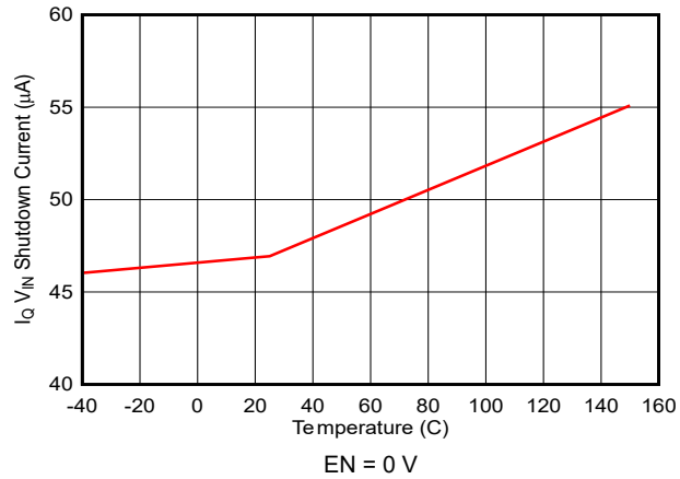
Figure 6-1. I_{Q\text{ VIN}} Shutdown Current vs Temperature
