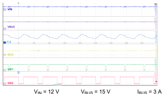
図 9-26. Buck-Boost Mode: Nominal V_{IN} , 3 A Load
