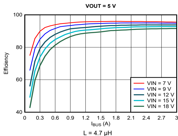
図 9-6. Efficiency vs Output Current ( I_{OUT} ), V_{OUT} = 5 V
