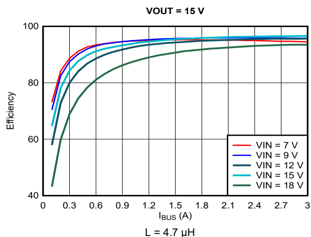
図 9-9. Efficiency vs Output Current ( I_{OUT} ), V_{OUT} = 15 V
