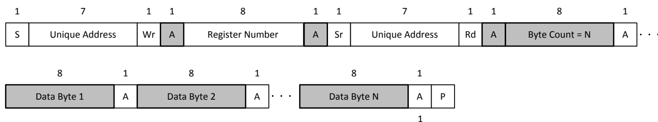
図 8-40. I²C Unique Address Read Register Protocol
