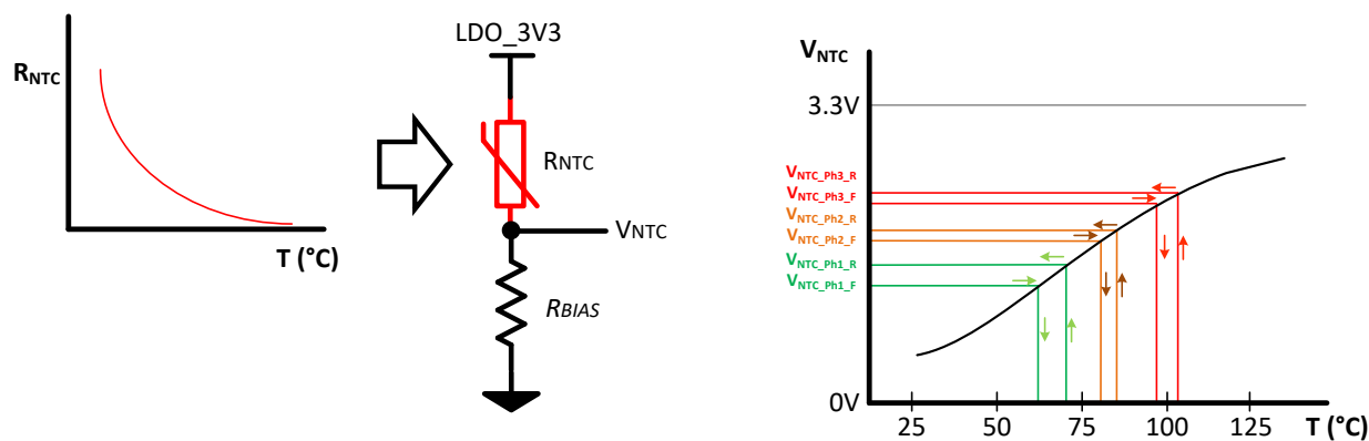
図 8-44. NTC Response Curve
