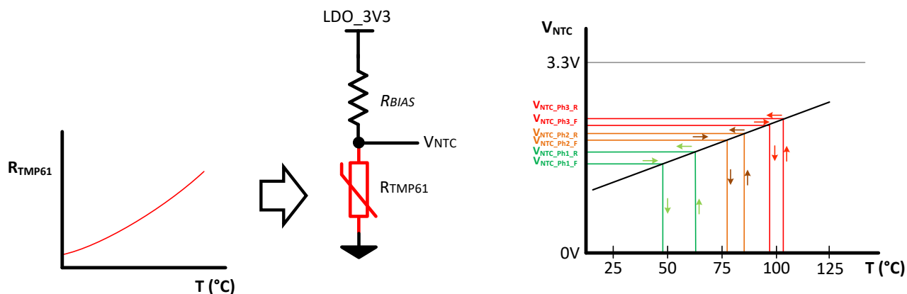
図 8-45. TMP61 PTC Response Curve
