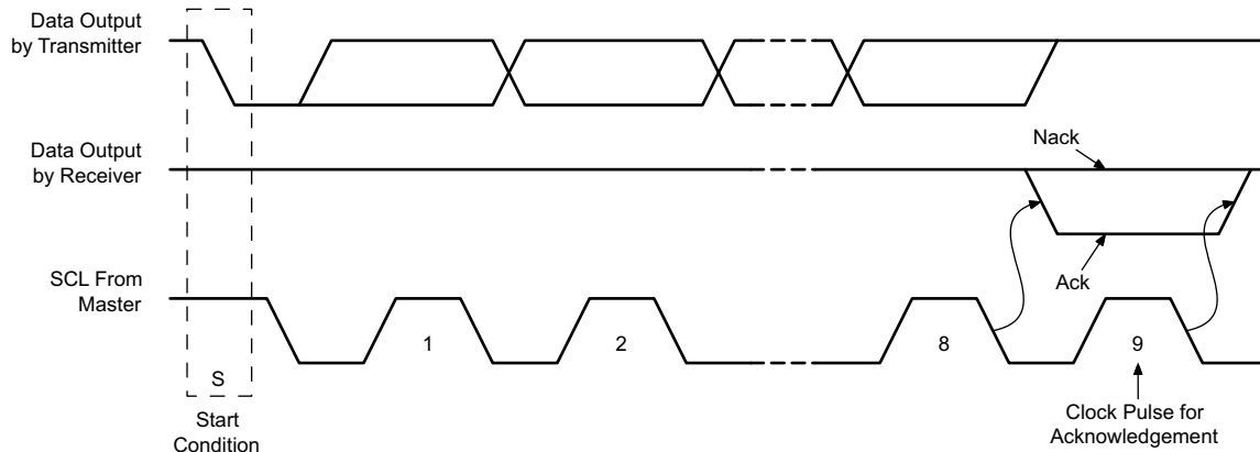
図 8-38. I 2 C Acknowledgment
