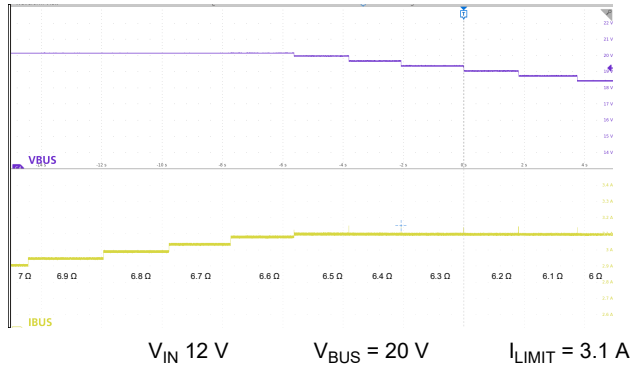
図 9-34. Current Limit: Stepped Resistive Load
