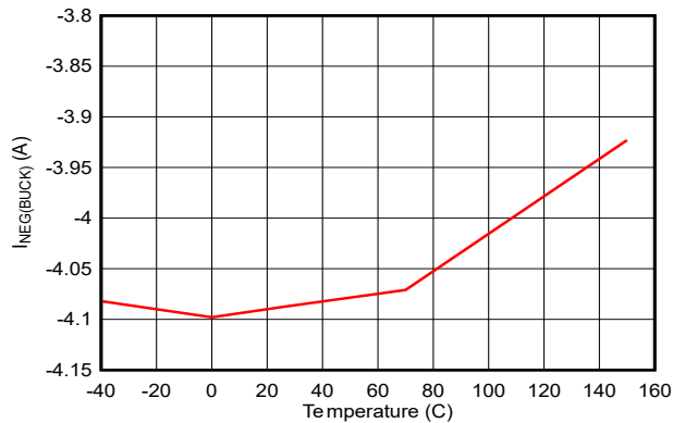
図 6-21. Buck Negative Current Limit vs Temperature
