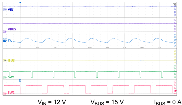
図 9-25. Buck-Boost Mode: Nominal V_{IN} , No Load
