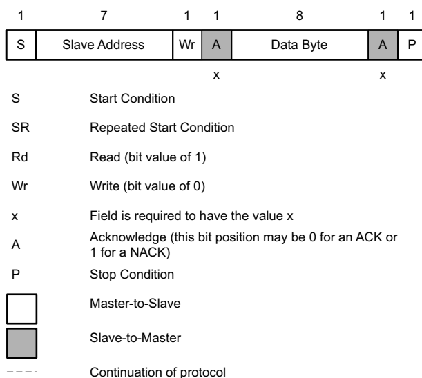
図 8-41. I²C Read/Write Protocol Key
