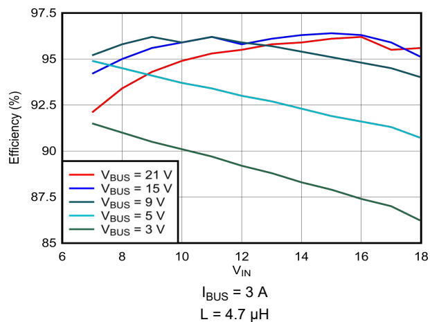
9-11. Efficiency vs Input Voltage
