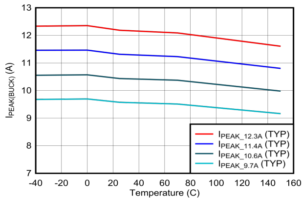
図 6-19. Buck Peak Current Limit vs Temperature (upper settings)
