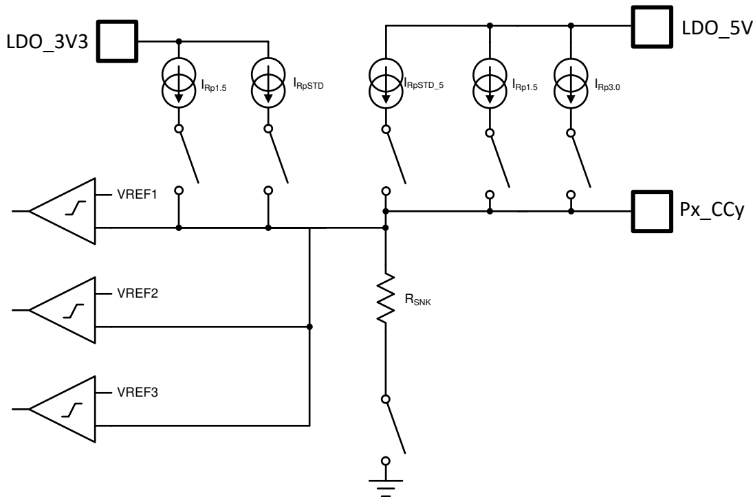
8-28. Plug and Orientation Detection Block
