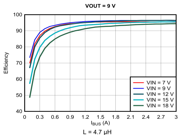
図 9-7. Efficiency vs Output Current ( I_{OUT} ), V_{OUT} = 9 V
