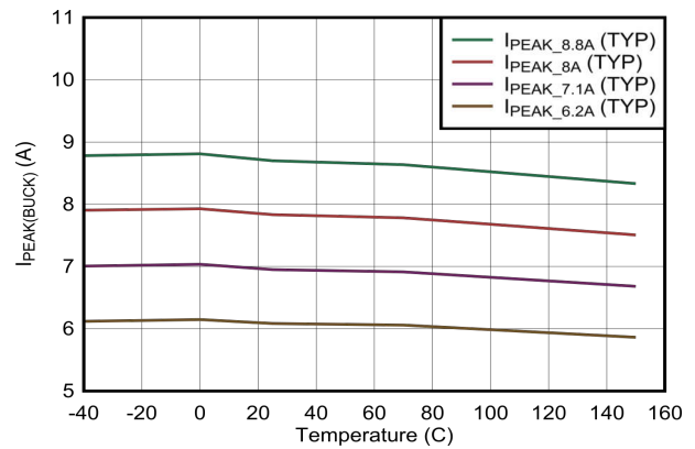
図 6-20. Buck Peak Current Limit vs Temperature (lower settings)
