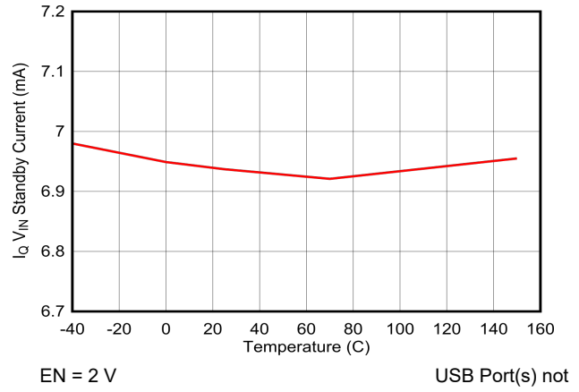
Figure 6-2. I_{Q\text{ VIN}} Standby Current vs Temperature
