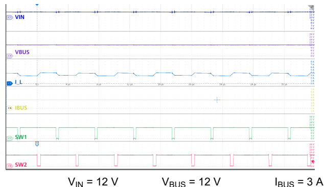
図 9-24. Buck-Boost Mode: V_{IN} = V_{BUS} , 3 A Load
