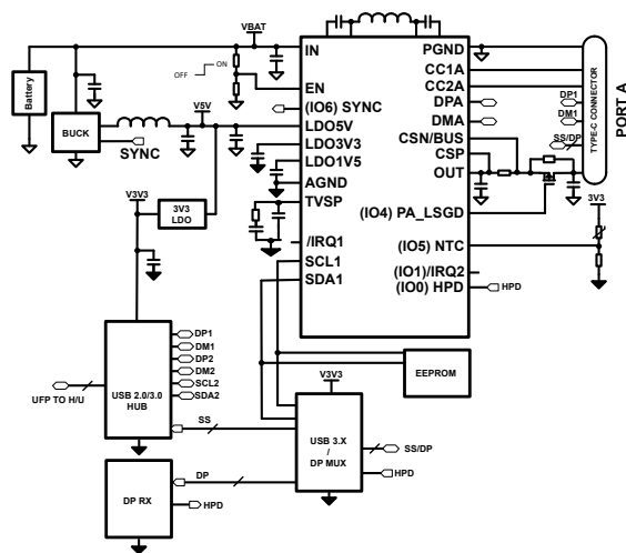
9-1. Simplified Single USB PD Charger with DisplayPort Alt Mode - MUX control with I2C
