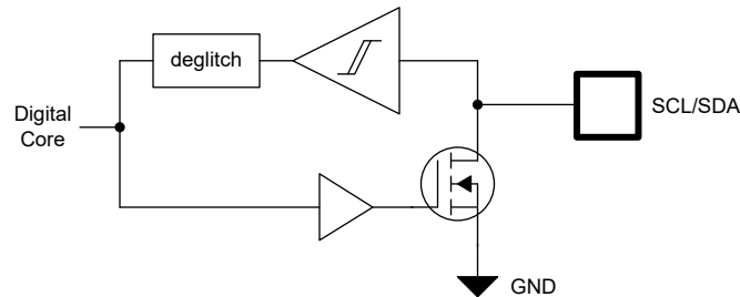
8-35. I 2 C Driver
