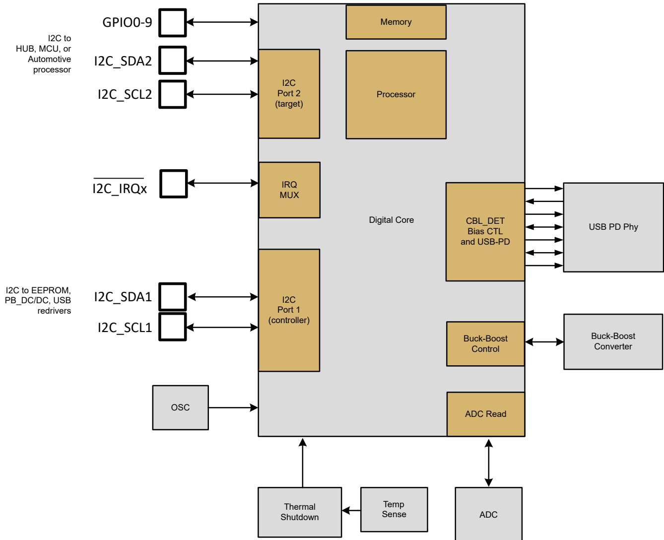
図 8-42. Digital Core Simplified Block Diagram
