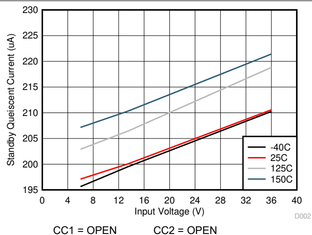
8-2. Standby Quiescent Current
