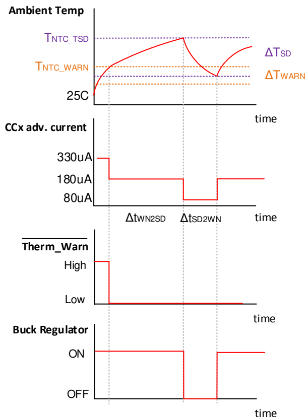
FIG 10-29. TPS25833-Q1 Behavior when Trigger NTC Threshold
