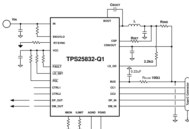
FIG 10-21. Buck Average Current Limit
