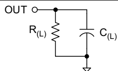
9-1. V_{\text{CONN}} Switch Rise-Fall Test Load Figure
