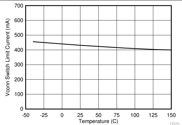
8-24. V CONN Switch Current Limit vs Junction Temperature
