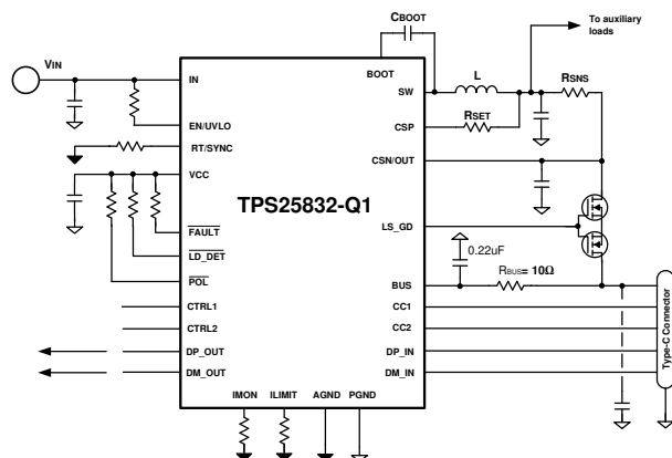
FIG 10-20. Current Limit with External MOSFET
