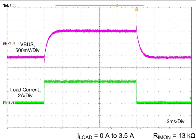
11-10. Load Transient with Cable Compensation
