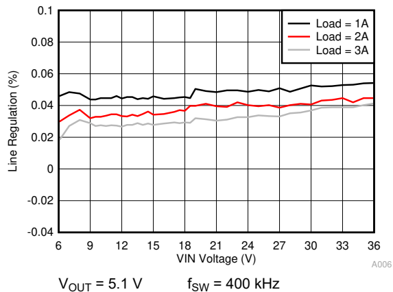
11-7. Line Regulation
