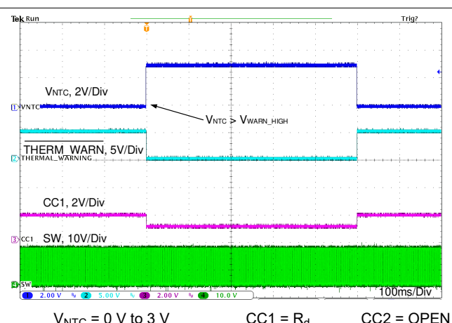
11-41. Thermal Sensing with NTC Behavior 1
