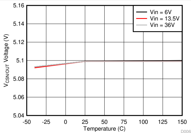
8-7. V_{CSN/OUT} Voltage vs Junction Temperature
