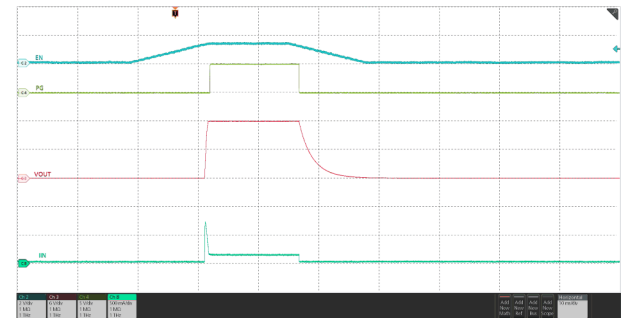
V IN = 12 V, C OUT = 22 μF, C dVdt = Open, V EN/UVLO ramped from 0 V → 1.4 V → 0 V
