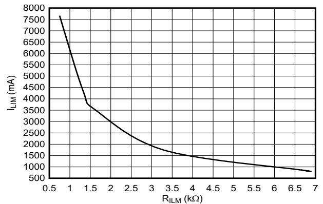
図 6-12. Overcurrent Threshold vs ILM Resistor
