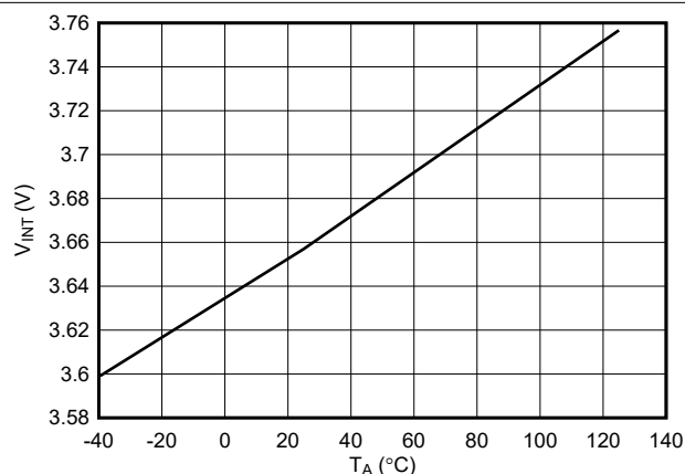
FIG 7-15. ITIMER Pin Internal Pullup Voltage Across Temperature
