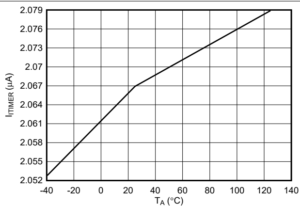
FIG 7-16. ITIMER Pin Discharge Current Across Temperature
