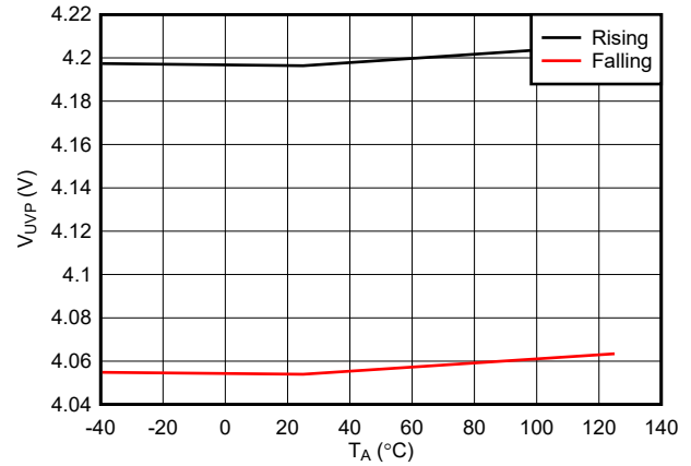
FIG 7-2. VDD Undervoltage Thresholds Across Temperature
