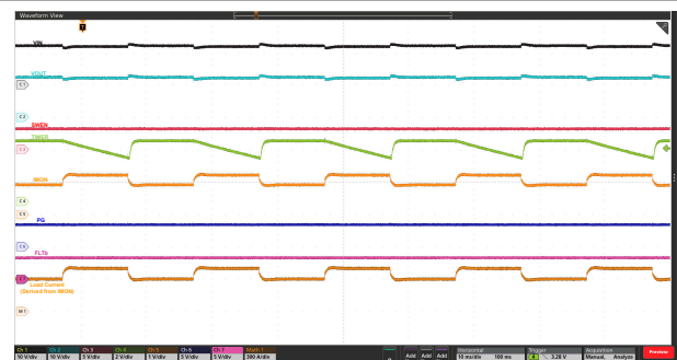
Figure 9-9. Transient Overload: V_{IN} = 12 V, C_{TIMER} = 22 nF, C_{LOAD} = 55 mF, R_{IMON} = 167 \Omega , R_{REF} = 40.2 k \Omega , and Load Current Stepped from 300 A to 400 A then 300 A within 10 ms
