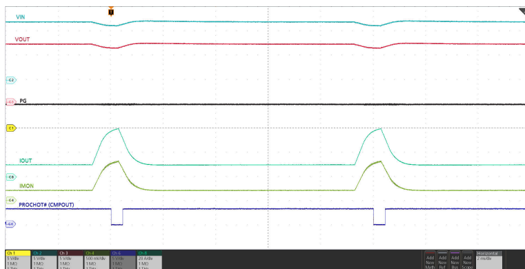
FIG 8-10. PROCHOT# Response Using Internal Comparator
