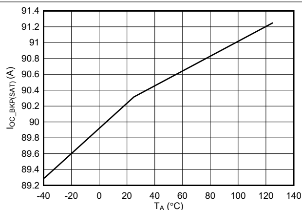
FIG 7-13. Backup Overcurrent Protection Threshold (Start-up) Accuracy
