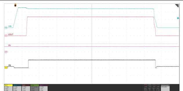
Figure 7-24. Power Up and Down Sequencing Using Input Supply
