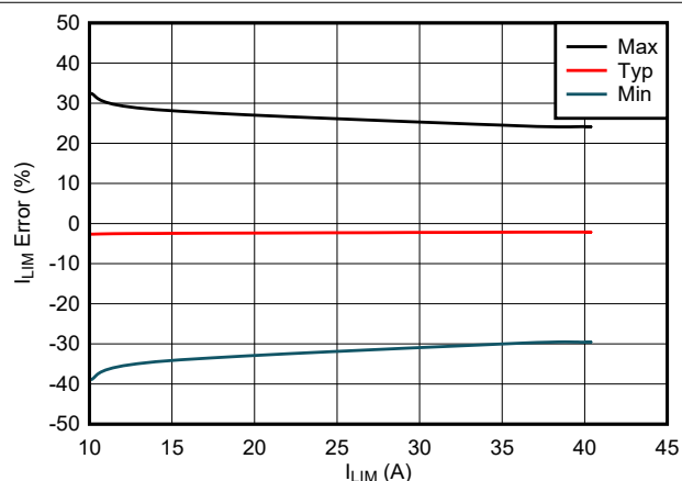
FIG 7-12. Start-up Overcurrent Protection Threshold (Current Limit) Accuracy
