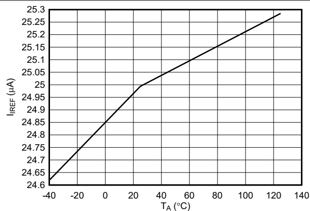
FIG 7-7. IREF Charging Current Across Temperature
