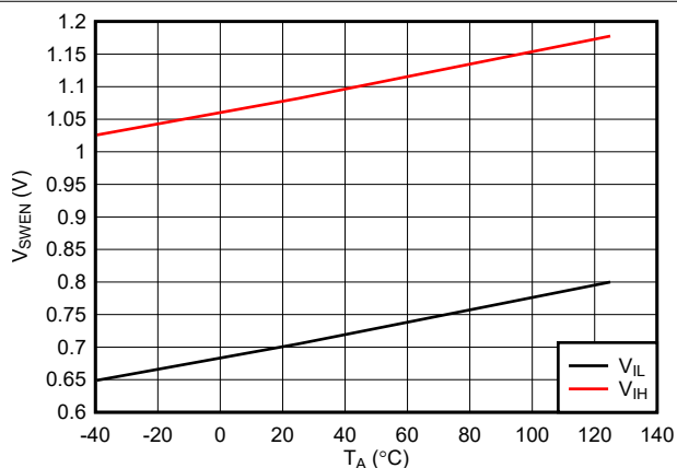
FIG 7-18. SWEN Pin Logic Thresholds Across Temperature
