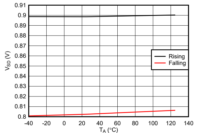
FIG 7-6. EN/UVLO Based Shutdown Falling Threshold Across Temperature
