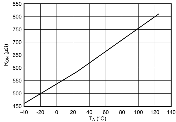
FIG 7-1. ON Resistance Across Temperature
