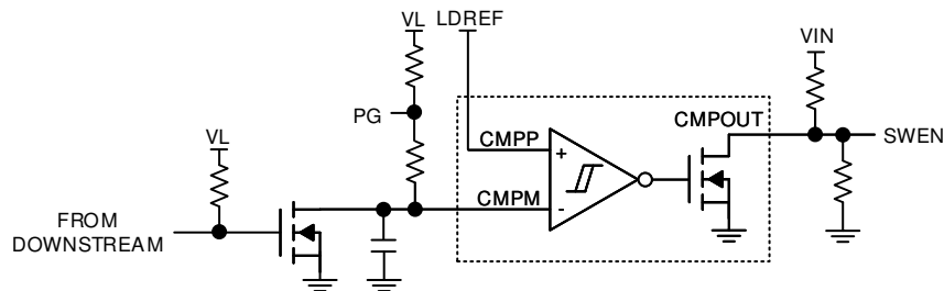
FIG 8-12. Load Handshake or Detect Timer Using Internal Comparator
