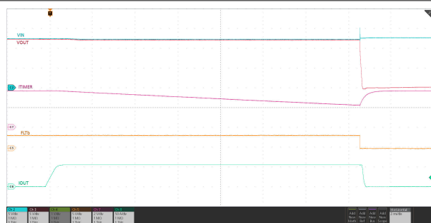
7-31. Overcurrent Protection Response (Circuit-Breaker)
