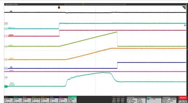
Figure 9-5. Start-up with EN/UVLO: V_{IN} = 12 V, EN/UVLO Stepped Up From 0 V to 3 V, C_{LOAD} = 55 mF, R_{LOAD(Start-up)} = 0.33 \Omega , C_{DVDT} = 33 nF, R_{REF} = 40.2 k \Omega , and R_{ILIM} on Each Device = 300 \Omega
