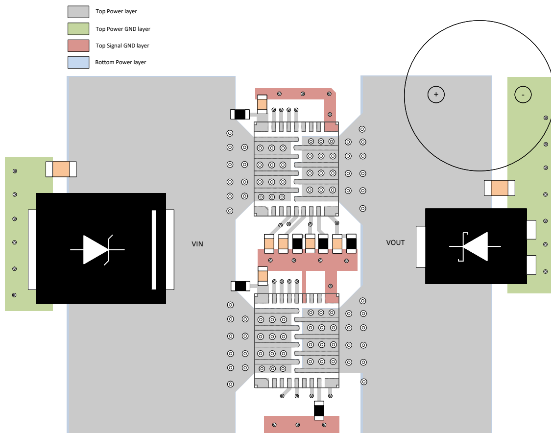
11-1. TPS25985x Two Parallel Devices Layout Example
