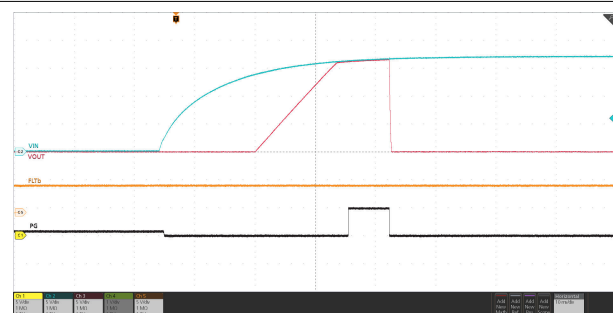
7-29. Input Overvoltage Protection Response
