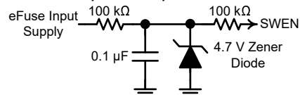
FIG 9-18. Zener Regulator Used as Pullup Supply for SWEN
