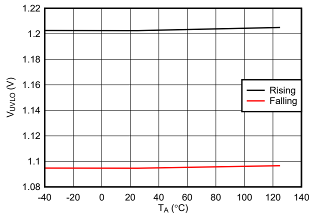
FIG 7-5. EN/UVLO Thresholds Across Temperature
