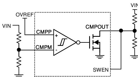
FIG 8-11. Fast Overvoltage Protection with Adjustable Threshold Using Internal Comparator
