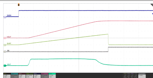
7-27. Inrush Current Control with Capacitive Load
