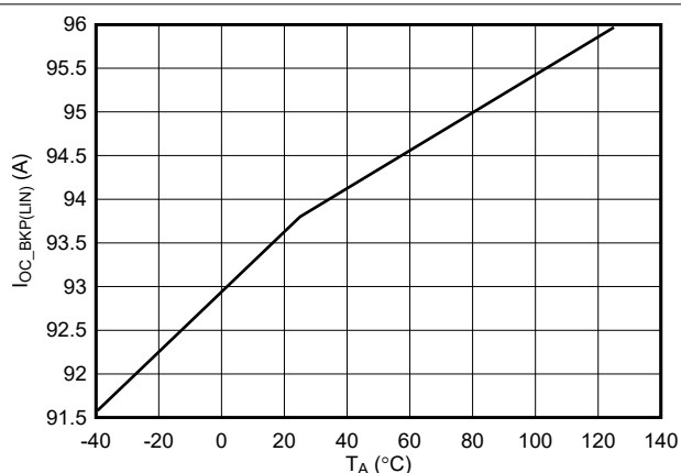
FIG 7-14. Backup Overcurrent Protection Threshold (Steady-State) Accuracy
