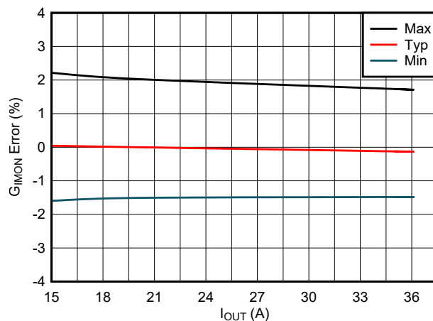
FIG 7-10. IMON Gain Accuracy Across Process and Temperature Corners
