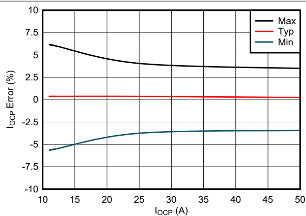
FIG 7-11. Steady-State Overcurrent Protection Threshold (Circuit-Breaker) Accuracy
