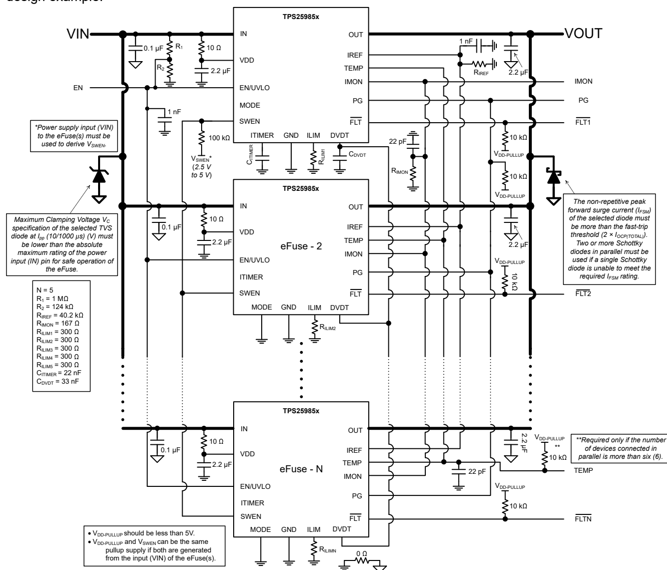
9-3. Application Schematic for a 12-V, 3.6-kW Power Path Protection Circuit
