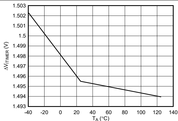
FIG 7-17. ITIMER Pin Discharge Differential Voltage Threshold Across Temperature
