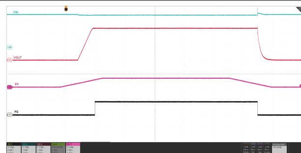
7-25. Power Up and Down Sequencing Using EN/UVLO Pin
