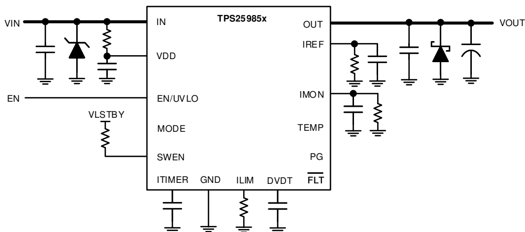
FIG 10-1. Circuit Implementation with Optional Protection Components
