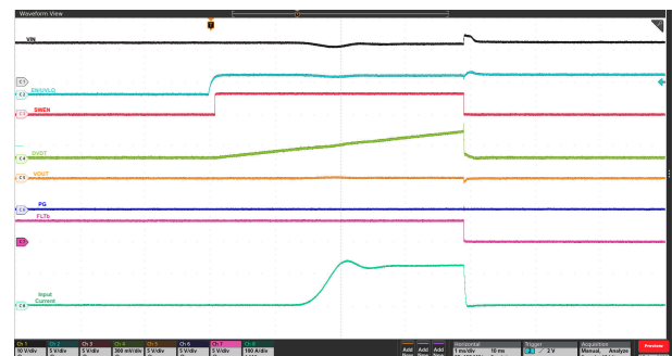
Figure 9-7. Power Up into Short: V_{IN} = 12 V, EN/UVLO Stepped Up From 0 V to 3 V, R_{REF} = 40.2 k \Omega , R_{ILIM} on Each Device = 300 \Omega , and OUT Shorted to GND
