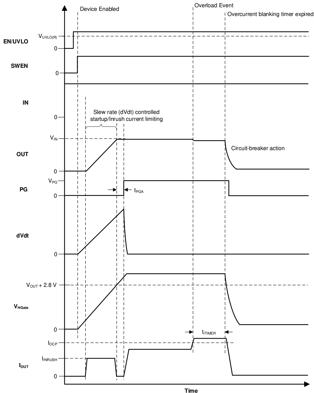
图 8-8. TPS25985x PG Timing Diagram
