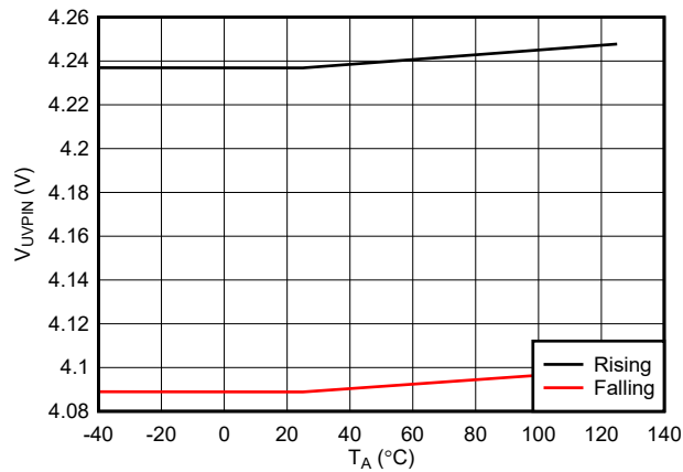
FIG 7-3. VIN Undervoltage Thresholds Across Temperature
