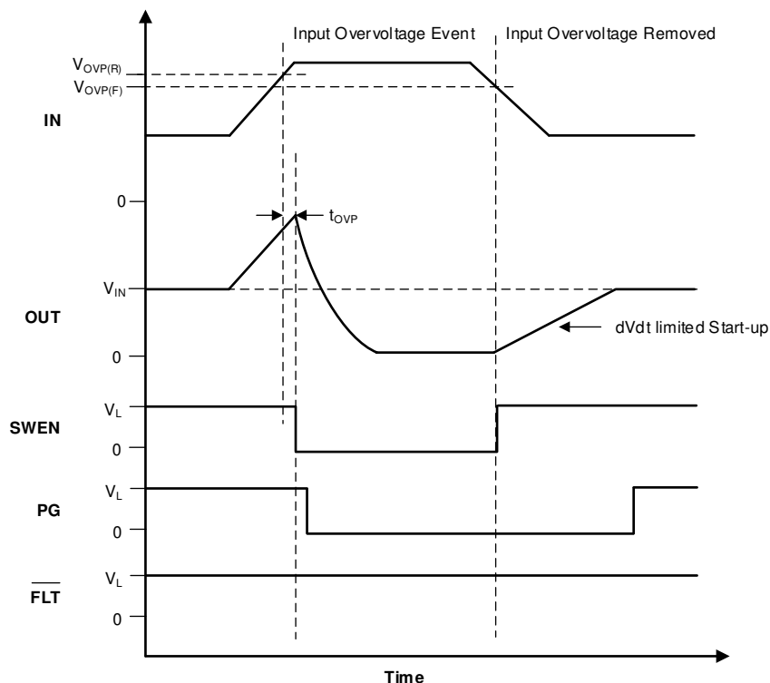
8-3. Input Overvoltage Protection Response
