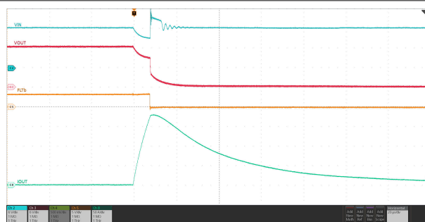
7-32. Short-Circuit Protection Response
