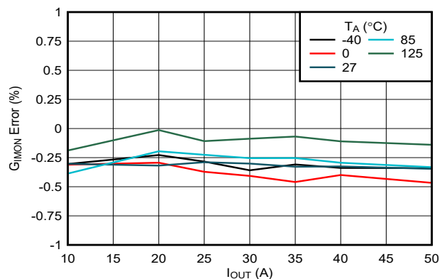
FIG 7-9. IMON Gain Accuracy Across Load and Temperature
