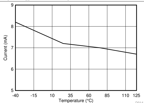
Figure 16. I_{OL,on}
