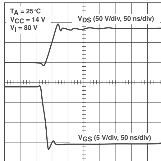
✎ 38. Drain-Source Voltage vs Gate-Source Voltage, at Turn-off, TPS2811 Driving an IRFD120 (Hex-2 Size)
