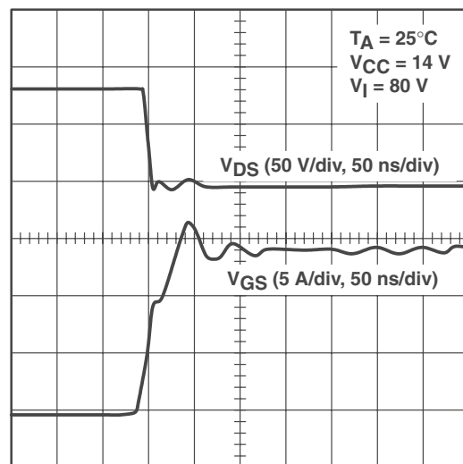
✎ 40. Drain-Source Voltage vs Gate-Source Voltage, at Turn-on, TPS2811 Driving an IRF530 (Hex-3 Size)
