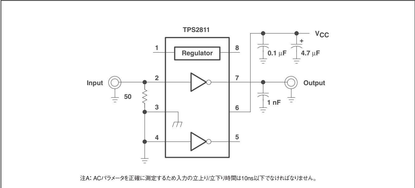
1. Test Circuit For Measurement of Switching Characteristics
