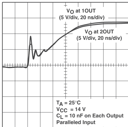
25. Voltage at 1OUT vs Voltage at 2OUT, Low-to-High Output Delay
