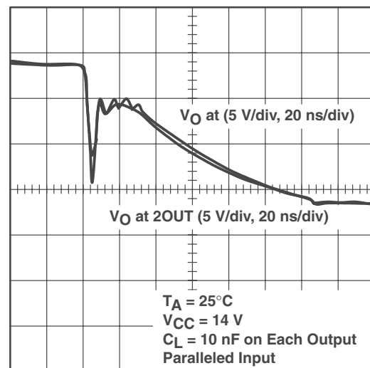
✎ 26. Voltage at 1OUT vs Voltage at 2OUT, High-to-Low Output Delay
