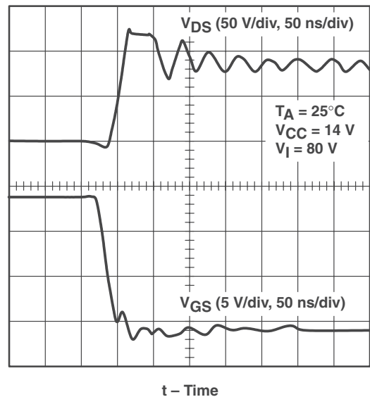
✎ 42. Drain-Source Voltage vs Gate-Source Voltage, at Turn-off, TPS2811 Driving an IRF530 (Hex-3 Size)
