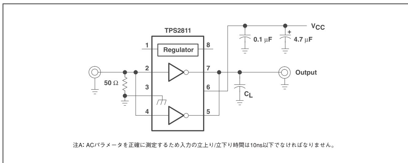
27. Test Circuit for Measuring Paralleled Switching Characteristics
