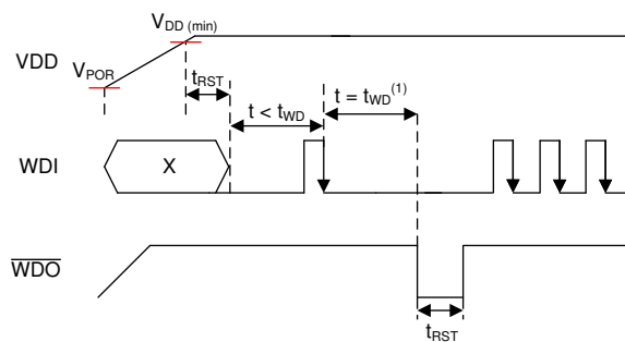
6-1. Timing Diagram
