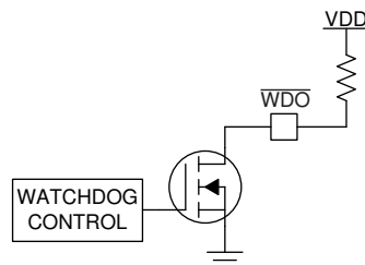
8-3. \overline{\text{WDO}} Open-Drain Configuration
