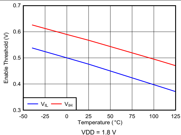
FIG 6-4. EN Threshold vs Temperature
