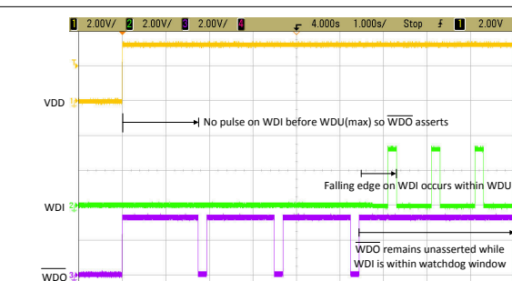
8-5. \overline{WDO} Fault Caused by missing WDI Pulses Followed by Correct Timing WDI Pulses
