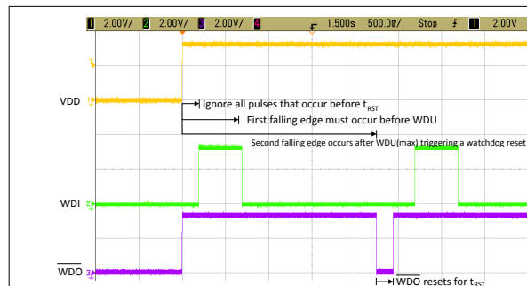
8-4. \overline{WDO} Fault Caused by WDI Pulse Arriving Too Late (After t_{WD(max)} )
