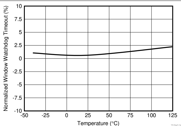
FIG 6-6. Normalized Watchdog Timeout ( t_{WD} ) Accuracy (SET1 = 1, CWD = NC)
