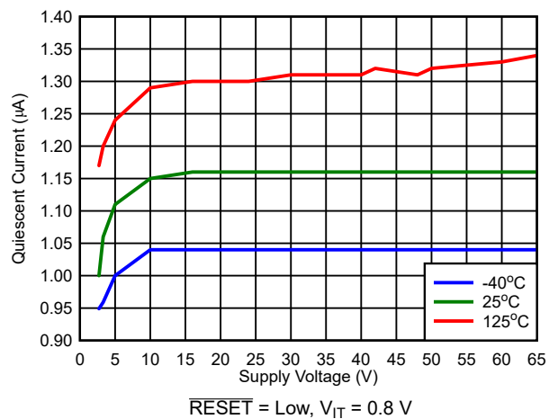
图 7-9. V_{DD} vs I_{DD} (RESET = Low, V_{IT} = 0.8\text{ V} )
