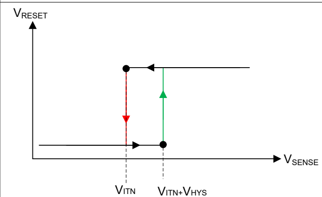
8-7. Hysteresis (Undervoltage Active-Low)
