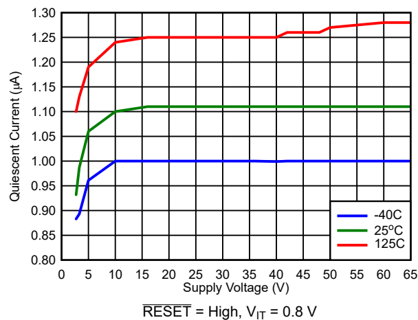
图 7-8. V_{DD} vs I_{DD} (RESET = High, V_{IT} = 0.8\text{ V} )
