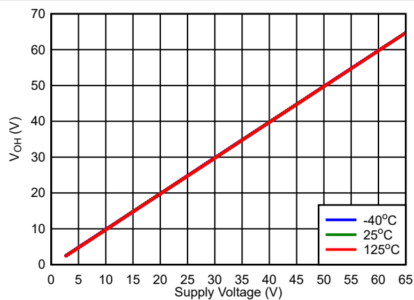
FIG 7-22. Push-Pull Active Low V_{OH} vs V_{DD}
