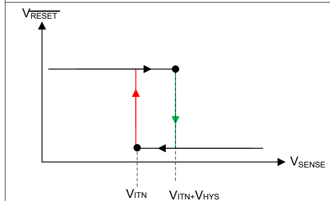
8-6. Hysteresis (Undervoltage Active-High)
