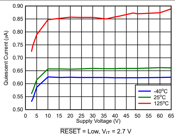
图 7-7. V_{DD} vs I_{DD} (RESET = Low, V_{IT} = 2.7\text{ V} )
