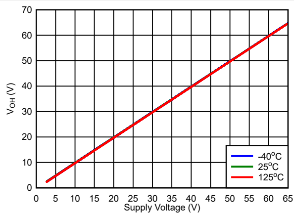
FIG 7-23. Push-Pull Active High V_{OH} vs V_{DD}
