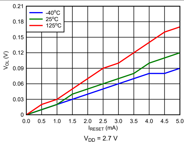
图 7-14. Open-Drain Active High V_{OL} vs I_{RESET}
