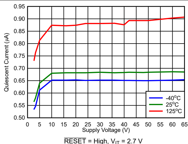
图 7-6. V_{DD} vs I_{DD} (RESET = High, V_{IT} = 2.7\text{ V} )
