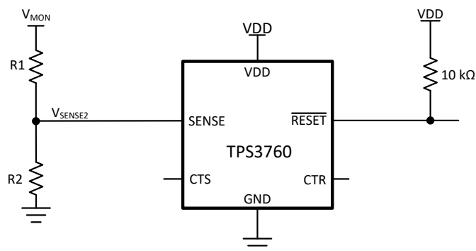
FIG 9-1. Adjustable Voltage Threshold with External Resistor Dividers
