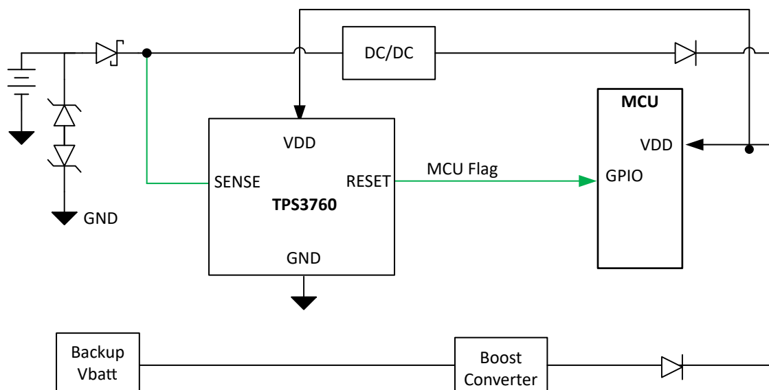
FIG 9-2. TPS3760 Overvoltage Supervisor with Direct Off-Battery Monitoring
