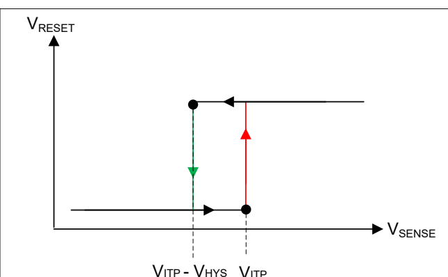
8-5. Hysteresis (Overvoltage Active-High)
