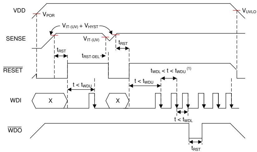
FIG 6-1. Timing Diagram
