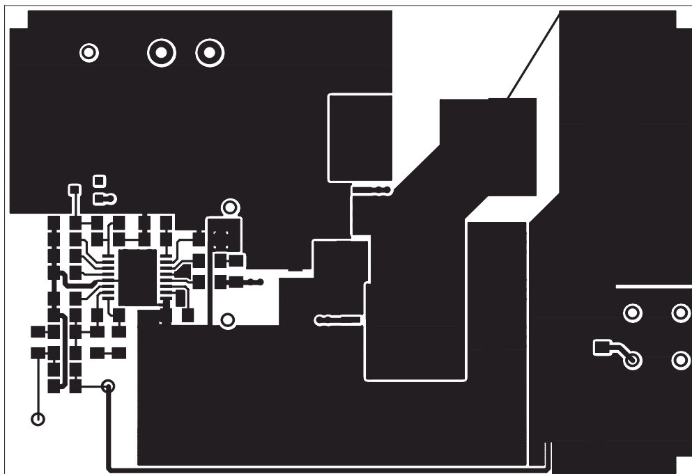
10-2. Top-Side Copper
