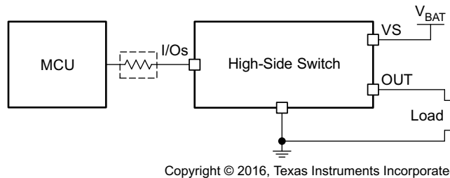
Figure 35. MCU I/O External Protection
