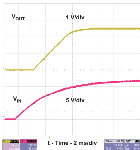
図 8-10. TPS54332 Start-Up
