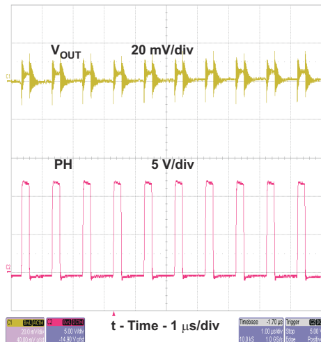
図 8-8. TPS54332 Output Ripple
