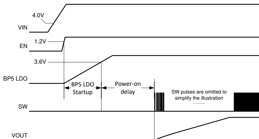
图 7-1. Start-up Sequence
