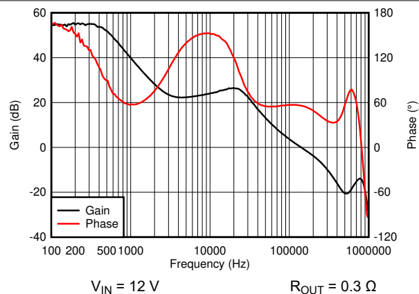
Figure 8-7. Bode Plot
