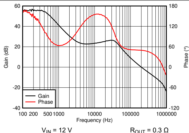
Figure 8-27. Bode Plot
