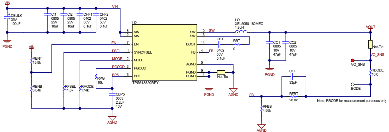
8-30. 12-V Input, 3.3-V Output, 1.0-MHz Schematic
