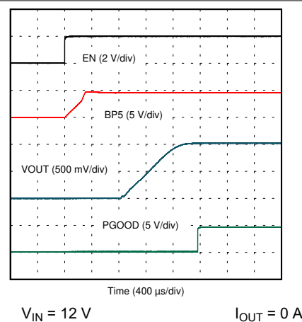
Figure 8-9. EN Start-up – Measuring BP5
