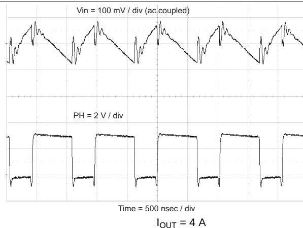
Figure 49. Input Ripple
