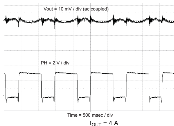
Figure 47. Output Ripple
