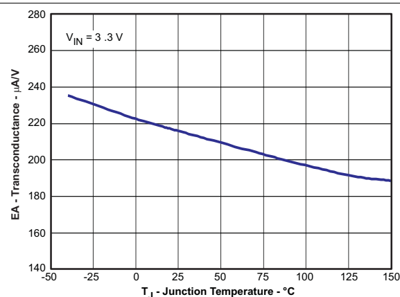
Figure 8. Transconductance vs Junction Temperature
