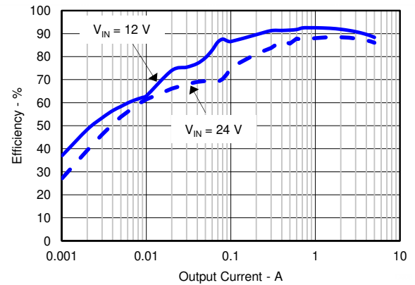
図 8-4. Low-Current Efficiency
