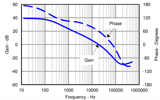
図 8-8. Loop Response
