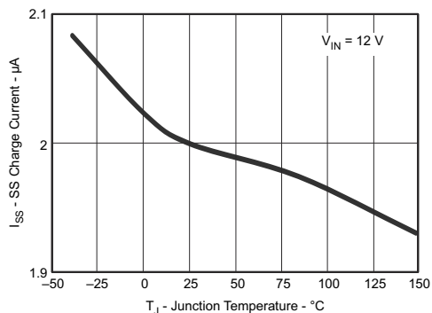
6-7. SS Charge Current vs Junction Temperature
