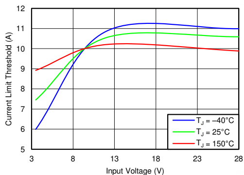
6-8. Current-Limit Threshold vs Input Voltage
