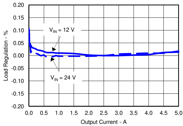
図 8-5. Load Regulation
