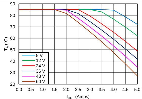
Figure 53. 5 V Outputs
