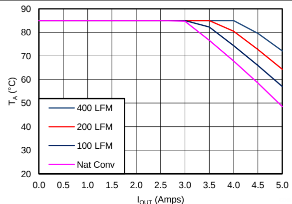
Figure 53. 5 V Outputs
